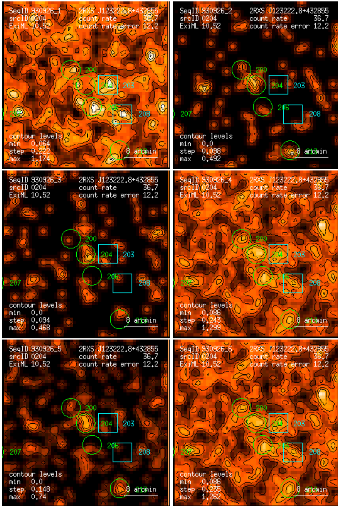
Figure 204: RASS 930926: detection 0204: band rate images, Gaussian filter: (1) PSPC channels 11 – 41, (2) 52 – 90, (3) 91 – 201, (4) 11 – 235, (5) 52 – 201, (6) 11 – 201. Broad band rates in counts/ks. Band rate contour levels in counts/ks/arcmin 2 .
