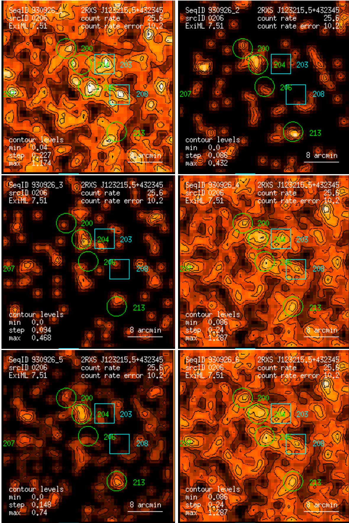
Figure 206: RASS 930926: detection 0206: band rate images, Gaussian filter: (1) PSPC channels 11 – 41, (2) 52 – 90, (3) 91 – 201, (4) 11 – 235, (5) 52 – 201, (6) 11 – 201. Broad band rates in counts/ks. Band rate contour levels in counts/ks/arcmin 2 .
