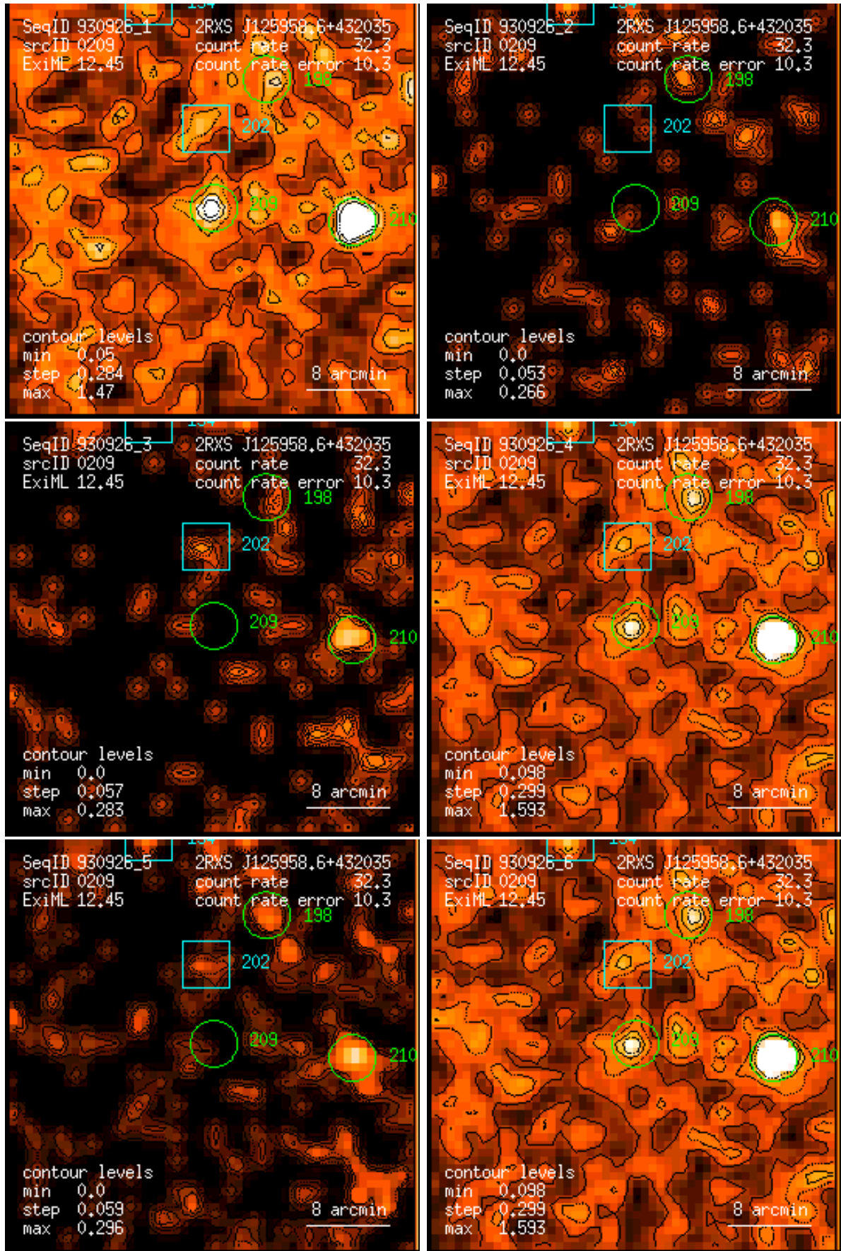
Figure 209: RASS 930926: detection 0209: band rate images, Gaussian filter: (1) PSPC channels 11 – 41, (2) 52 – 90, (3) 91 – 201, (4) 11 – 235, (5) 52 – 201, (6) 11 – 201. Broad band rates in counts/ks. Band rate contour levels in counts/ks/arcmin 2 .
