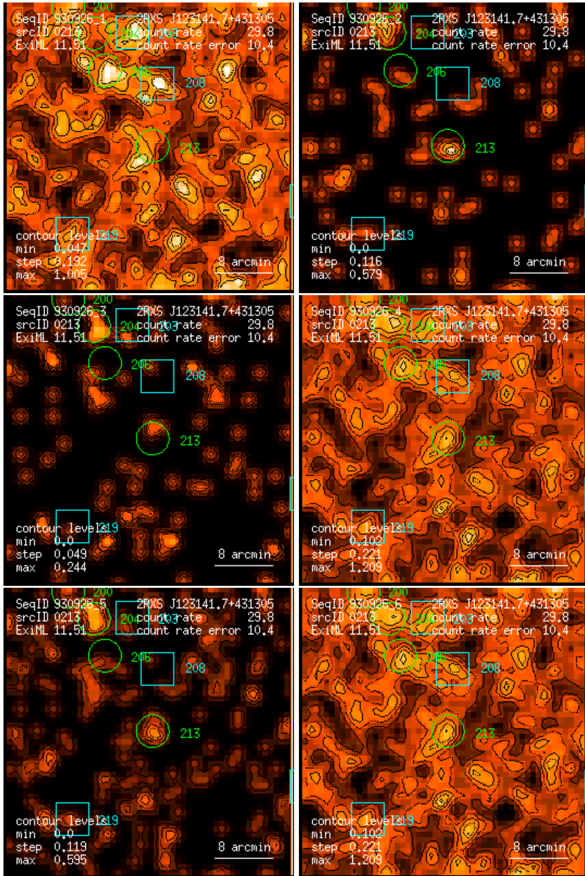
Figure 213: RASS 930926: detection 0213: band rate images, Gaussian filter: (1) PSPC channels 11 – 41, (2) 52 – 90, (3) 91 – 201, (4) 11 – 235, (5) 52 – 201, (6) 11 – 201. Broad band rates in counts/ks. Band rate contour levels in counts/ks/arcmin 2 .
