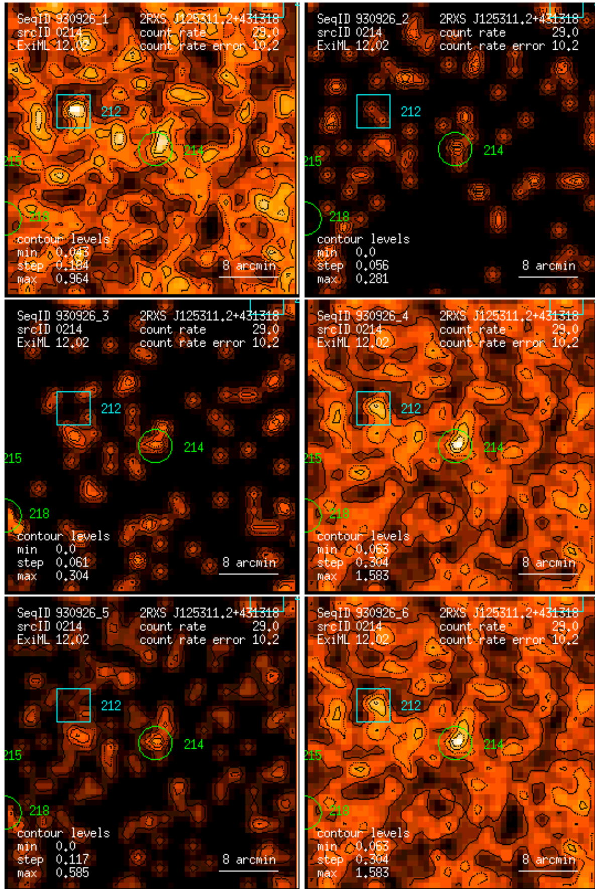
Figure 214: RASS 930926: detection 0214: band rate images, Gaussian filter: (1) PSPC channels 11 – 41, (2) 52 – 90, (3) 91 – 201, (4) 11 – 235, (5) 52 – 201, (6) 11 – 201. Broad band rates in counts/ks. Band rate contour levels in counts/ks/arcmin 2 .
