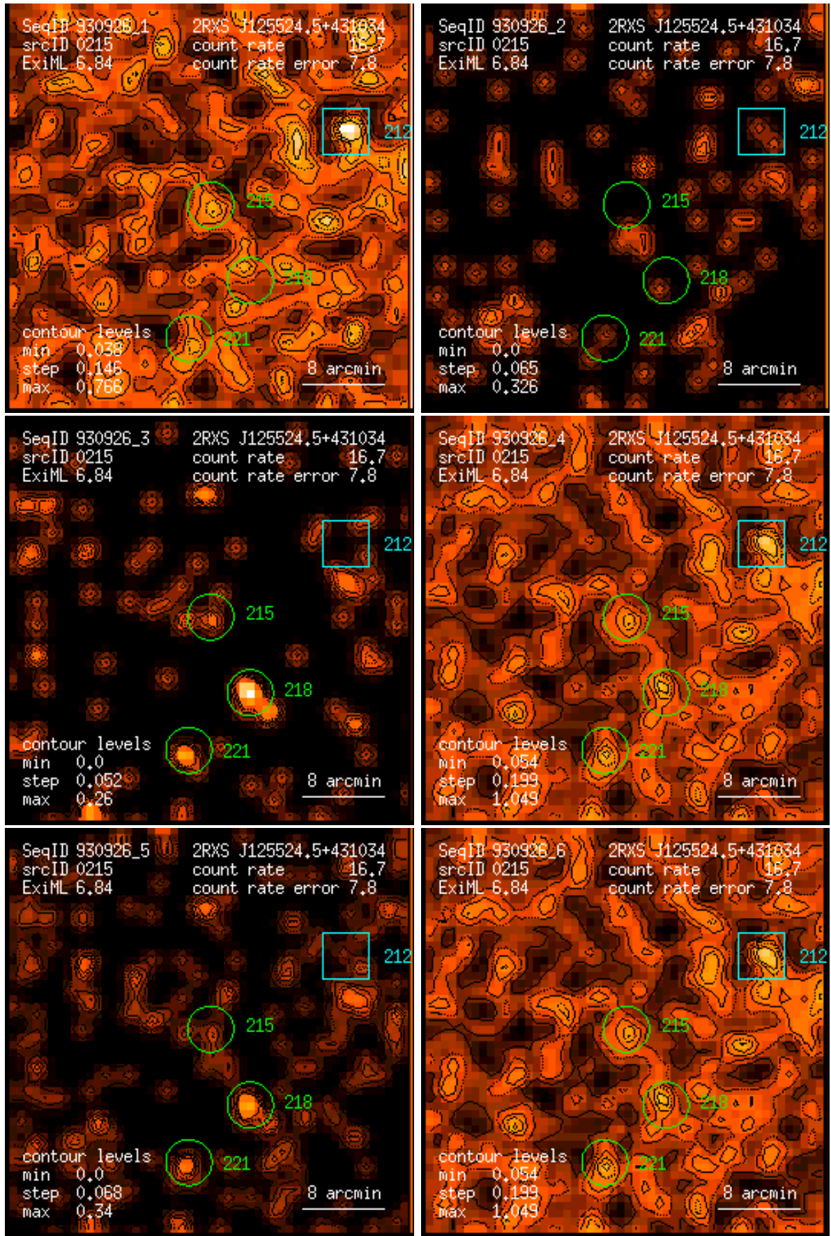
Figure 215: RASS 930926: detection 0215: band rate images, Gaussian filter: (1) PSPC channels 11 – 41, (2) 52 – 90, (3) 91 – 201, (4) 11 – 235, (5) 52 – 201, (6) 11 – 201. Broad band rates in counts/ks. Band rate contour levels in counts/ks/arcmin 2 .
