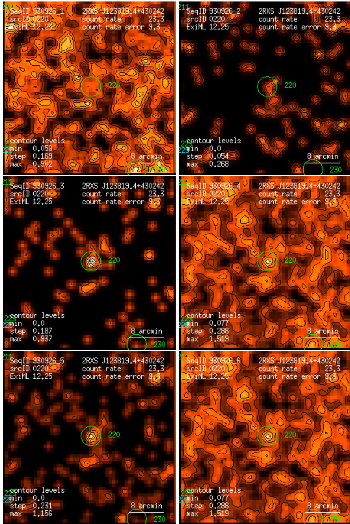
Figure 220: RASS 930926: detection 0220: band rate images, Gaussian filter: (1) PSPC channels 11 – 41, (2) 52 – 90, (3) 91 – 201, (4) 11 – 235, (5) 52 – 201, (6) 11 – 201. Broad band rates in counts/ks. Band rate contour levels in counts/ks/arcmin 2 .
