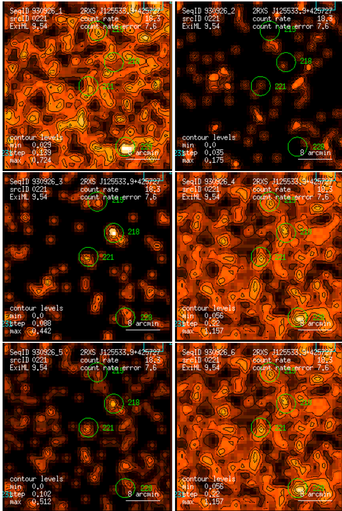
Figure 221: RASS 930926: detection 0221: band rate images, Gaussian filter: (1) PSPC channels 11 – 41, (2) 52 – 90, (3) 91 – 201, (4) 11 – 235, (5) 52 – 201, (6) 11 – 201. Broad band rates in counts/ks. Band rate contour levels in counts/ks/arcmin 2 .
