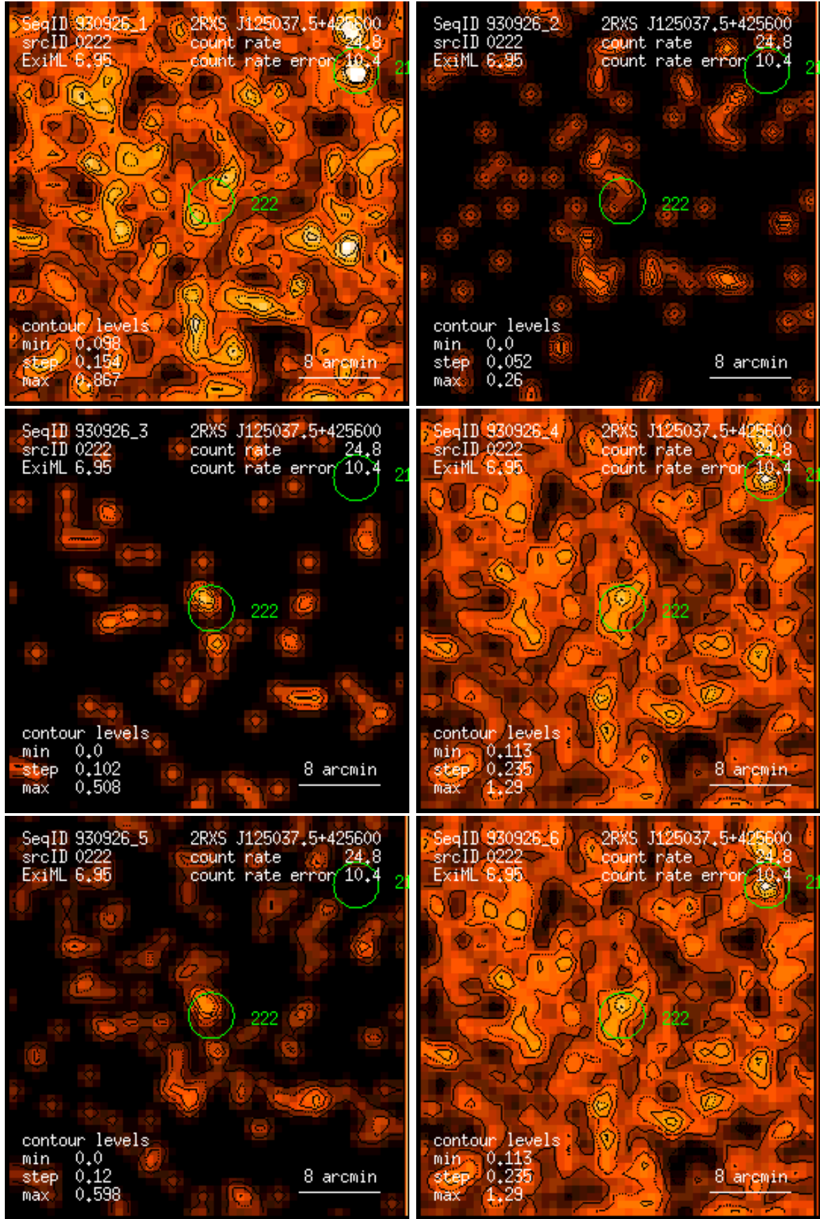
Figure 222: RASS 930926: detection 0222: band rate images, Gaussian filter: (1) PSPC channels 11 – 41, (2) 52 – 90, (3) 91 – 201, (4) 11 – 235, (5) 52 – 201, (6) 11 – 201. Broad band rates in counts/ks. Band rate contour levels in counts/ks/arcmin 2 .
