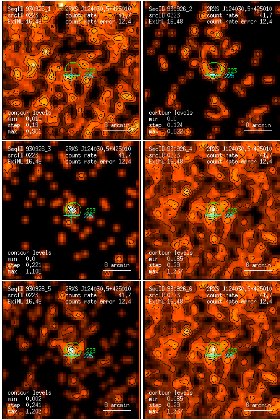
Figure 223: RASS 930926: detection 0223: band rate images, Gaussian filter: (1) PSPC channels 11 – 41, (2) 52 – 90, (3) 91 – 201, (4) 11 – 235, (5) 52 – 201, (6) 11 – 201. Broad band rates in counts/ks. Band rate contour levels in counts/ks/arcmin 2 .
