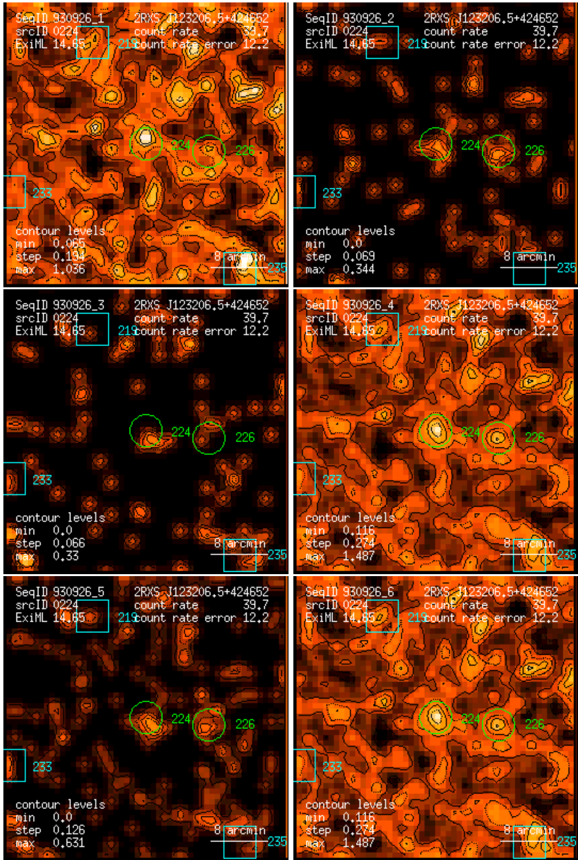
Figure 224: RASS 930926: detection 0224: band rate images, Gaussian filter: (1) PSPC channels 11 – 41, (2) 52 – 90, (3) 91 – 201, (4) 11 – 235, (5) 52 – 201, (6) 11 – 201. Broad band rates in counts/ks. Band rate contour levels in counts/ks/arcmin 2 .
