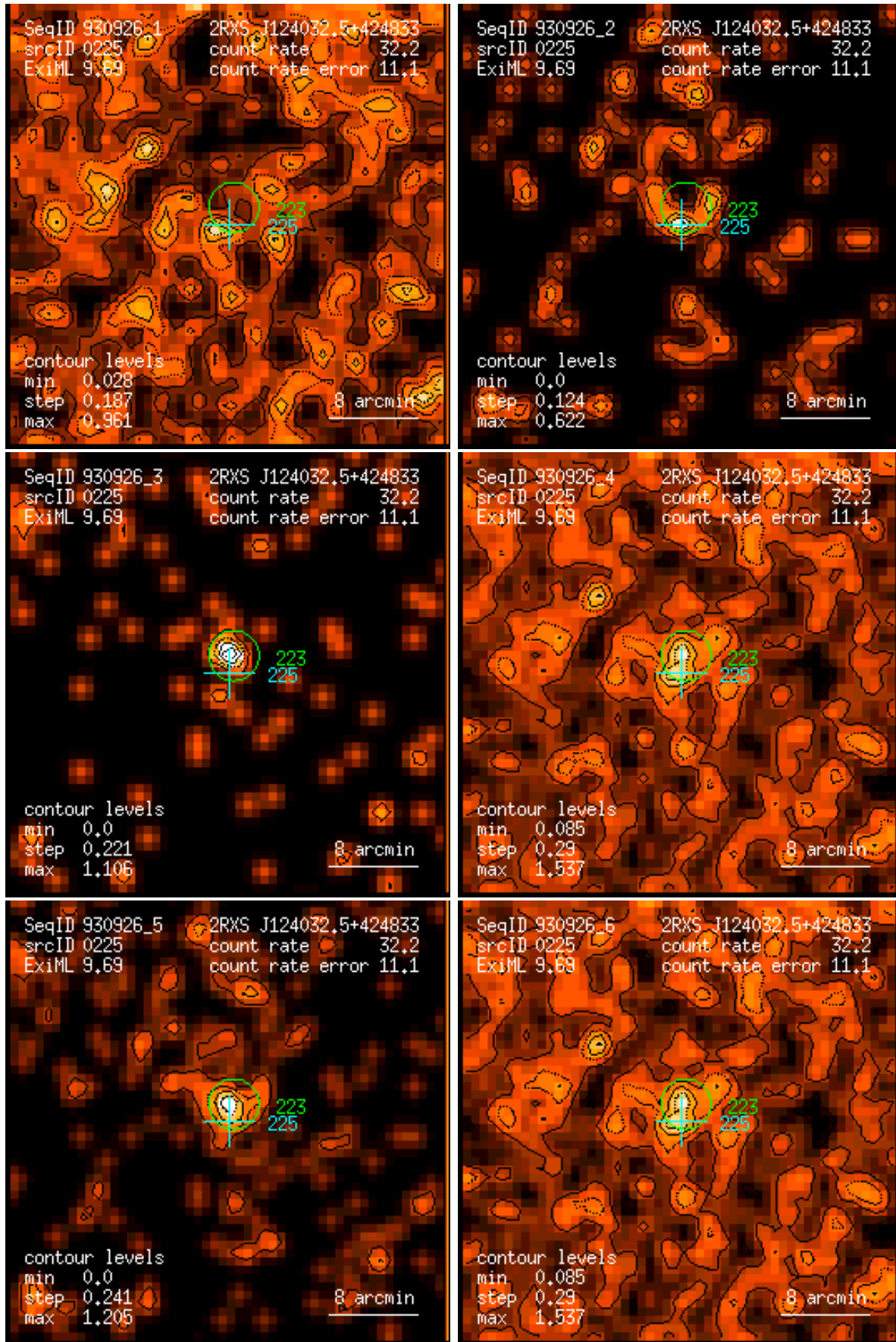
Figure 225: RASS 930926: detection 0225: band rate images, Gaussian filter: (1) PSPC channels 11 – 41, (2) 52 – 90, (3) 91 – 201, (4) 11 – 235, (5) 52 – 201, (6) 11 – 201. Broad band rates in counts/ks. Band rate contour levels in counts/ks/arcmin 2 .
