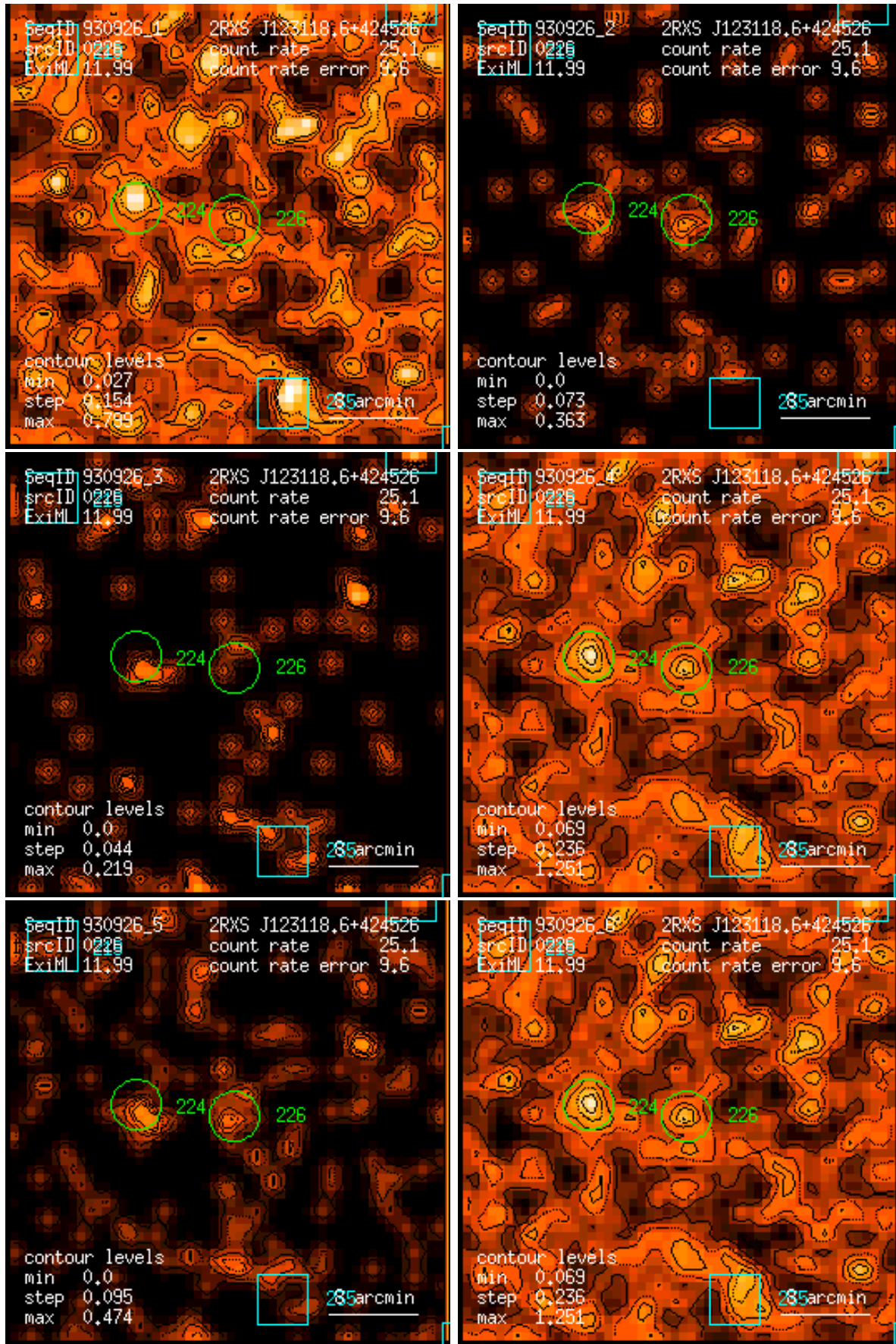
Figure 226: RASS 930926: detection 0226: band rate images, Gaussian filter: (1) PSPC channels 11 – 41, (2) 52 – 90, (3) 91 – 201, (4) 11 – 235, (5) 52 – 201, (6) 11 – 201. Broad band rates in counts/ks. Band rate contour levels in counts/ks/arcmin 2 .
