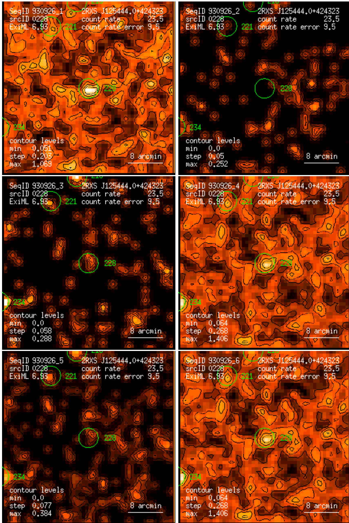
Figure 228: RASS 930926: detection 0228: band rate images, Gaussian filter: (1) PSPC channels 11 – 41, (2) 52 – 90, (3) 91 – 201, (4) 11 – 235, (5) 52 – 201, (6) 11 – 201. Broad band rates in counts/ks. Band rate contour levels in counts/ks/arcmin 2 .
