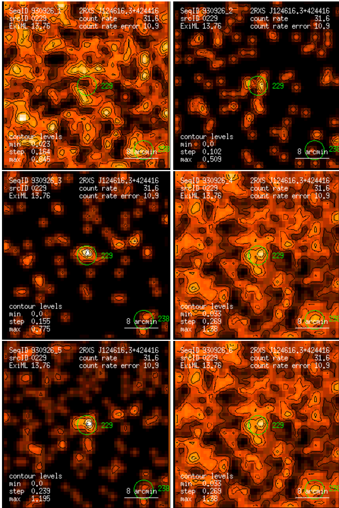
Figure 229: RASS 930926: detection 0229: band rate images, Gaussian filter: (1) PSPC channels 11 – 41, (2) 52 – 90, (3) 91 – 201, (4) 11 – 235, (5) 52 – 201, (6) 11 – 201. Broad band rates in counts/ks. Band rate contour levels in counts/ks/arcmin 2 .
