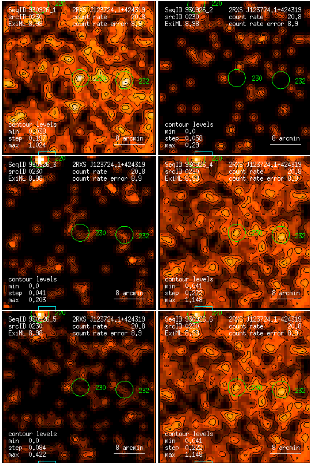
Figure 230: RASS 930926: detection 0230: band rate images, Gaussian filter: (1) PSPC channels 11 – 41, (2) 52 – 90, (3) 91 – 201, (4) 11 – 235, (5) 52 – 201, (6) 11 – 201. Broad band rates in counts/ks. Band rate contour levels in counts/ks/arcmin 2 .
