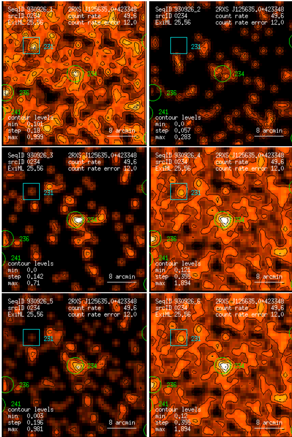
Figure 234: RASS 930926: detection 0234: band rate images, Gaussian filter: (1) PSPC channels 11 – 41, (2) 52 – 90, (3) 91 – 201, (4) 11 – 235, (5) 52 – 201, (6) 11 – 201. Broad band rates in counts/ks. Band rate contour levels in counts/ks/arcmin 2 .
