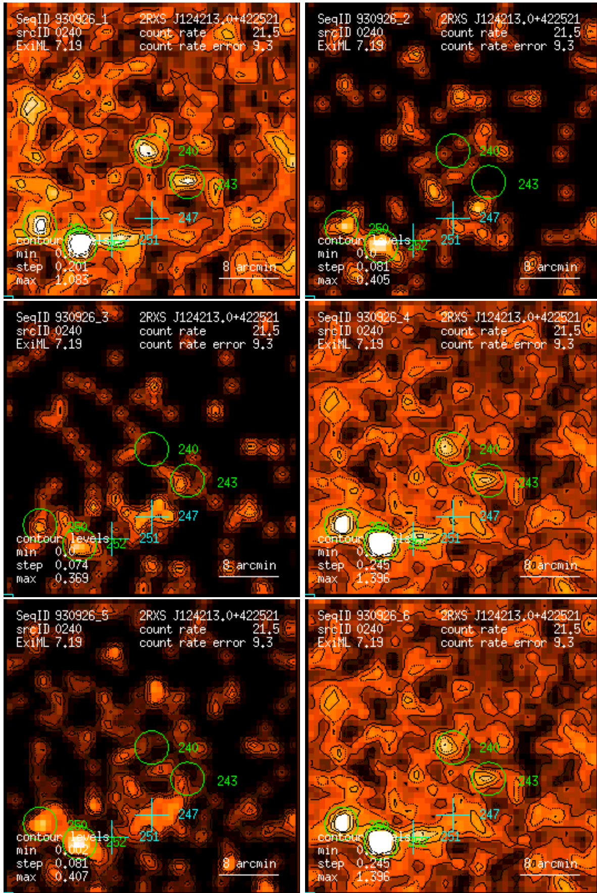
Figure 240: RASS 930926: detection 0240: band rate images, Gaussian filter: (1) PSPC channels 11 – 41, (2) 52 – 90, (3) 91 – 201, (4) 11 – 235, (5) 52 – 201, (6) 11 – 201. Broad band rates in counts/ks. Band rate contour levels in counts/ks/arcmin 2 .
