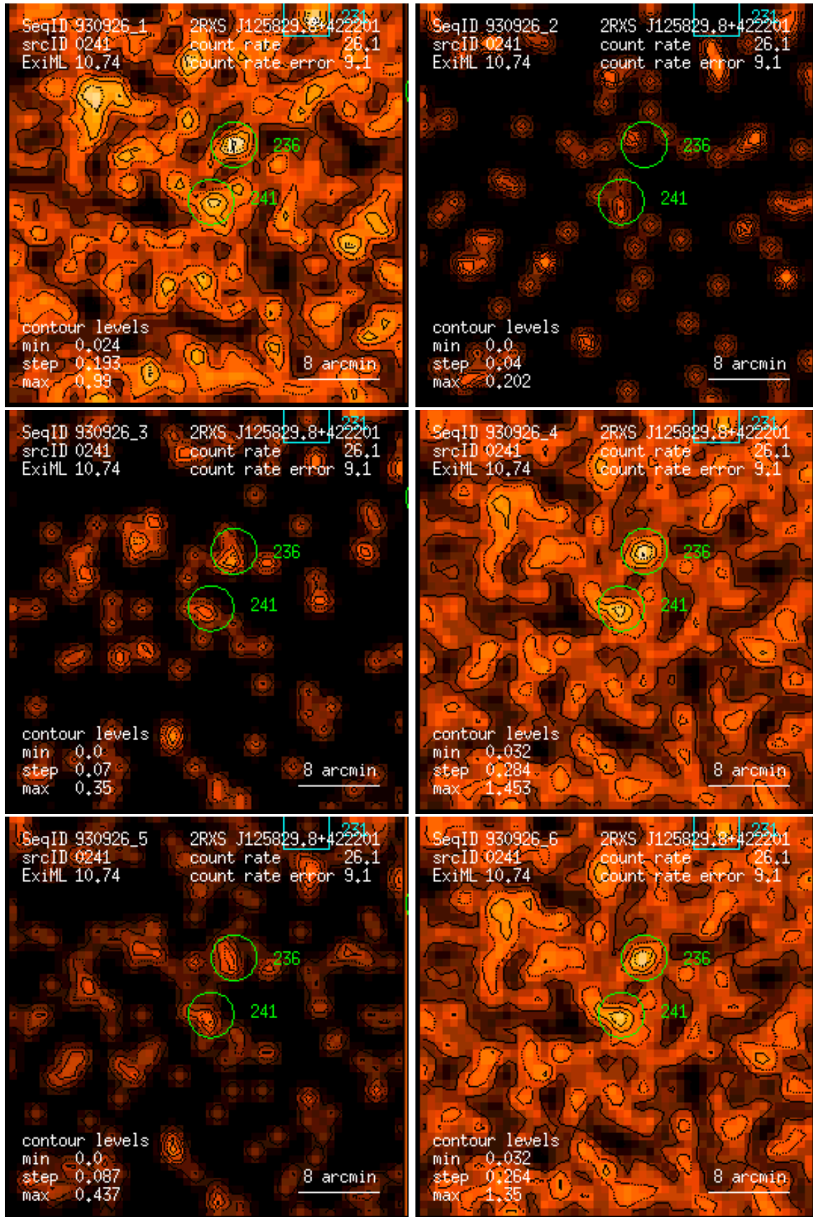
Figure 241: RASS 930926: detection 0241: band rate images, Gaussian filter: (1) PSPC channels 11 – 41, (2) 52 – 90, (3) 91 – 201, (4) 11 – 235, (5) 52 – 201, (6) 11 – 201. Broad band rates in counts/ks. Band rate contour levels in counts/ks/arcmin 2 .
