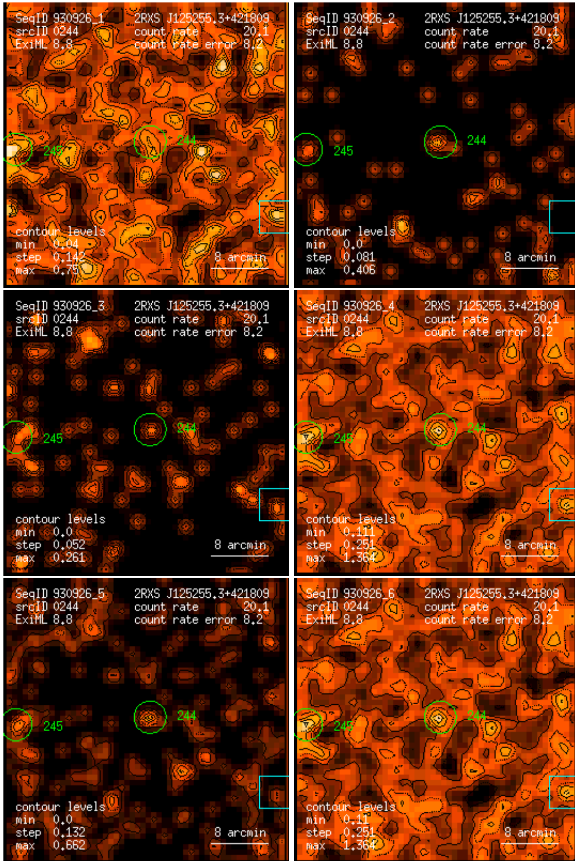
Figure 244: RASS 930926: detection 0244: band rate images, Gaussian filter: (1) PSPC channels 11 – 41, (2) 52 – 90, (3) 91 – 201, (4) 11 – 235, (5) 52 – 201, (6) 11 – 201. Broad band rates in counts/ks. Band rate contour levels in counts/ks/arcmin 2 .
