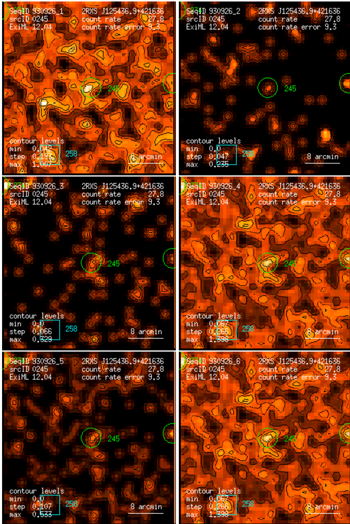
Figure 245: RASS 930926: detection 0245: band rate images, Gaussian filter: (1) PSPC channels 11 – 41, (2) 52 – 90, (3) 91 – 201, (4) 11 – 235, (5) 52 – 201, (6) 11 – 201. Broad band rates in counts/ks. Band rate contour levels in counts/ks/arcmin 2 .
