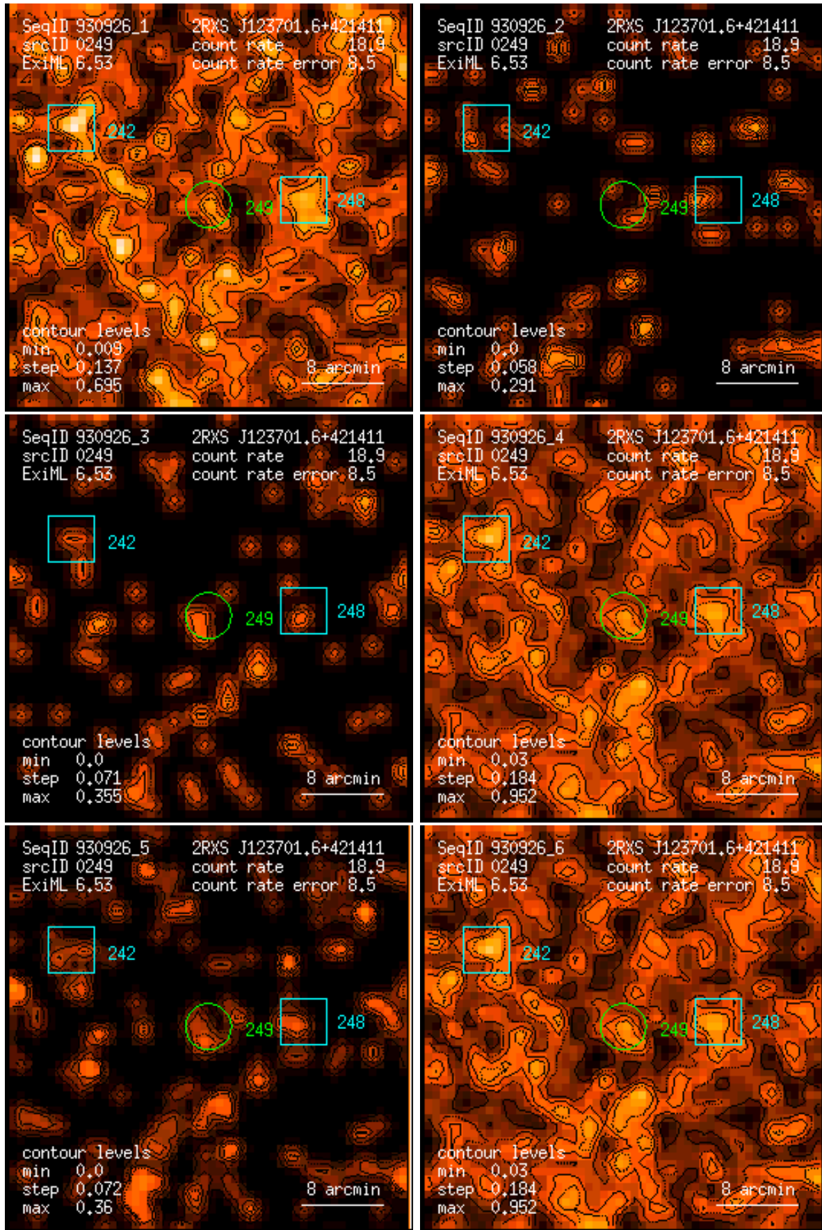
Figure 249: RASS 930926: detection 0249: band rate images, Gaussian filter: (1) PSPC channels 11 – 41, (2) 52 – 90, (3) 91 – 201, (4) 11 – 235, (5) 52 – 201, (6) 11 – 201. Broad band rates in counts/ks. Band rate contour levels in counts/ks/arcmin 2 .
