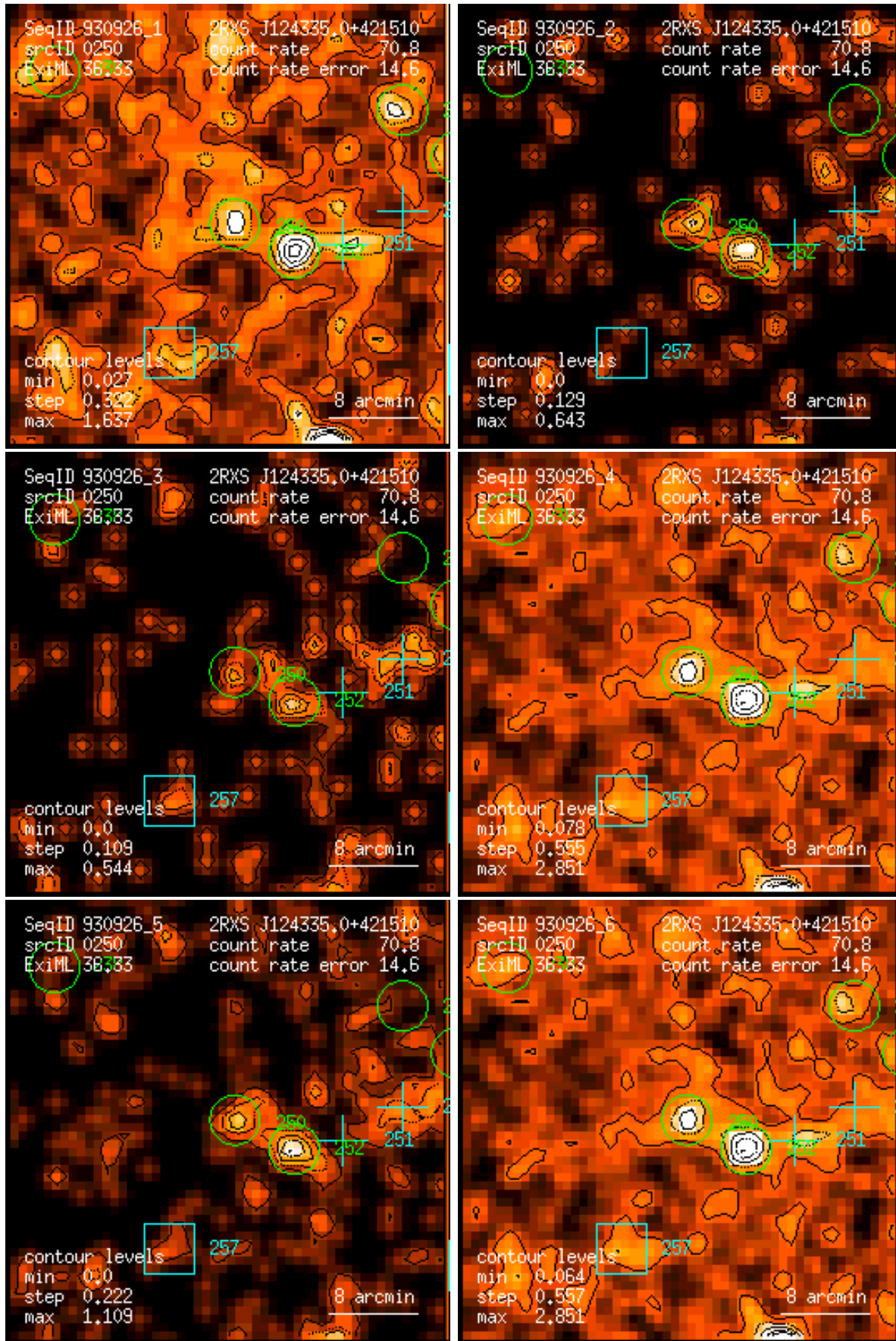
Figure 250: RASS 930926: detection 0250: band rate images, Gaussian filter: (1) PSPC channels 11 – 41, (2) 52 – 90, (3) 91 – 201, (4) 11 – 235, (5) 52 – 201, (6) 11 – 201. Broad band rates in counts/ks. Band rate contour levels in counts/ks/arcmin 2 .
