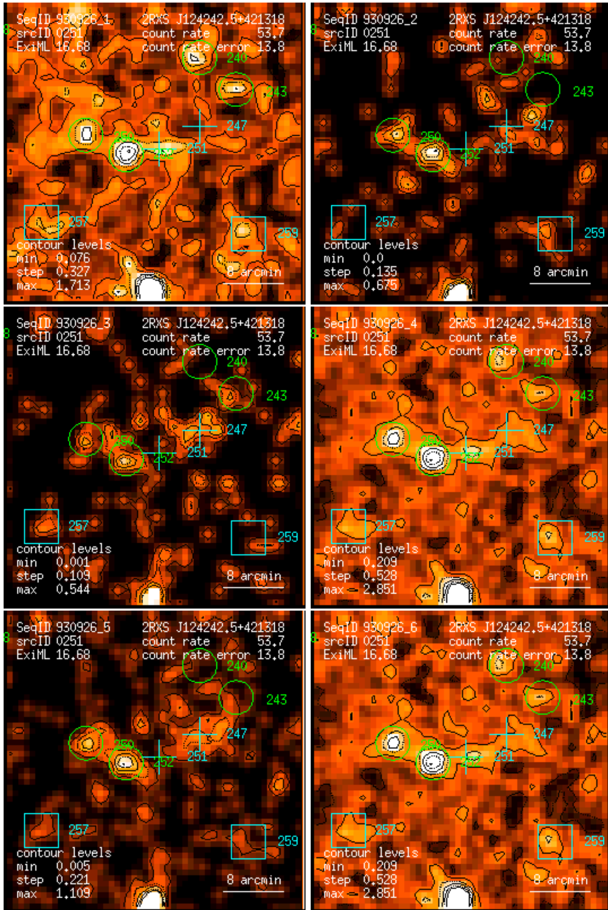
Figure 251: RASS 930926: detection 0251: band rate images, Gaussian filter: (1) PSPC channels 11 – 41, (2) 52 – 90, (3) 91 – 201, (4) 11 – 235, (5) 52 – 201, (6) 11 – 201. Broad band rates in counts/ks. Band rate contour levels in counts/ks/arcmin 2 .
