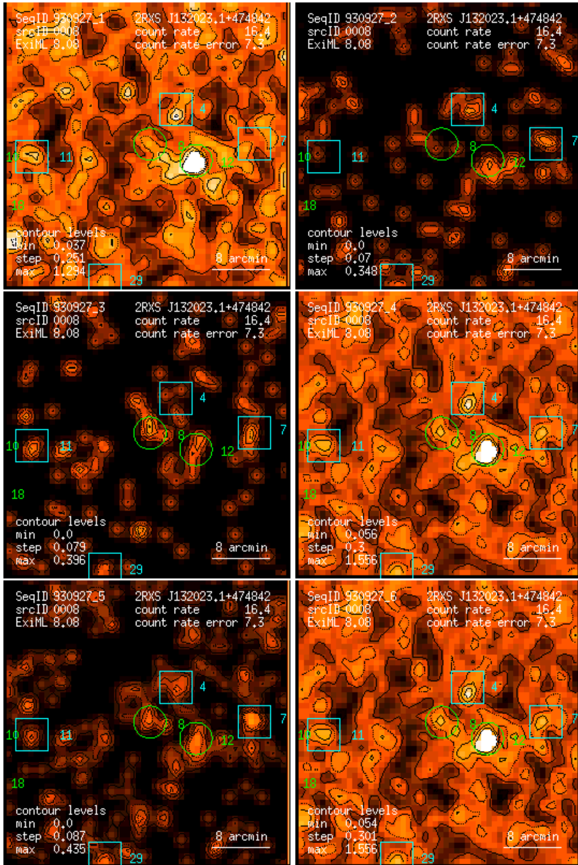
Figure 8: RASS 930927: detection 0008: band rate images, Gaussian filter: (1) PSPC channels 11 – 41, (2) 52 – 90, (3) 91 – 201, (4) 11 – 235, (5) 52 – 201, (6) 11 – 201. Broad band rates in counts/ks. Band rate contour levels in counts/ks/arcmin 2 .
