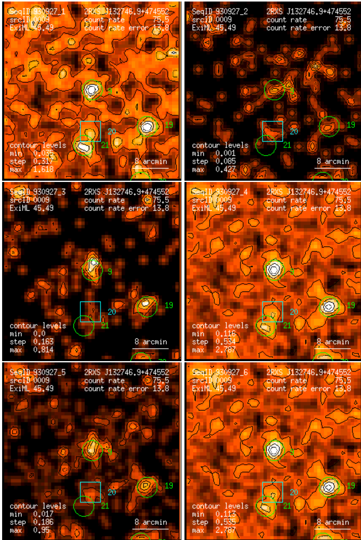
Figure 9: RASS 930927: detection 0009: band rate images, Gaussian filter: (1) PSPC channels 11 – 41, (2) 52 – 90, (3) 91 – 201, (4) 11 – 235, (5) 52 – 201, (6) 11 – 201. Broad band rates in counts/ks. Band rate contour levels in counts/ks/arcmin 2 .
