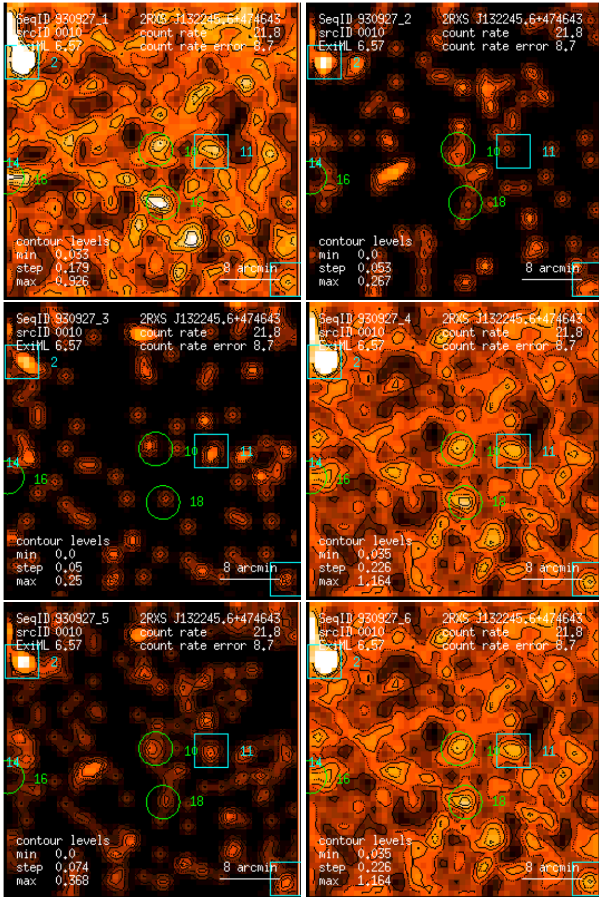
Figure 10: RASS 930927: detection 0010: band rate images, Gaussian filter: (1) PSPC channels 11 – 41, (2) 52 – 90, (3) 91 – 201, (4) 11 – 235, (5) 52 – 201, (6) 11 – 201. Broad band rates in counts/ks. Band rate contour levels in counts/ks/arcmin 2 .
