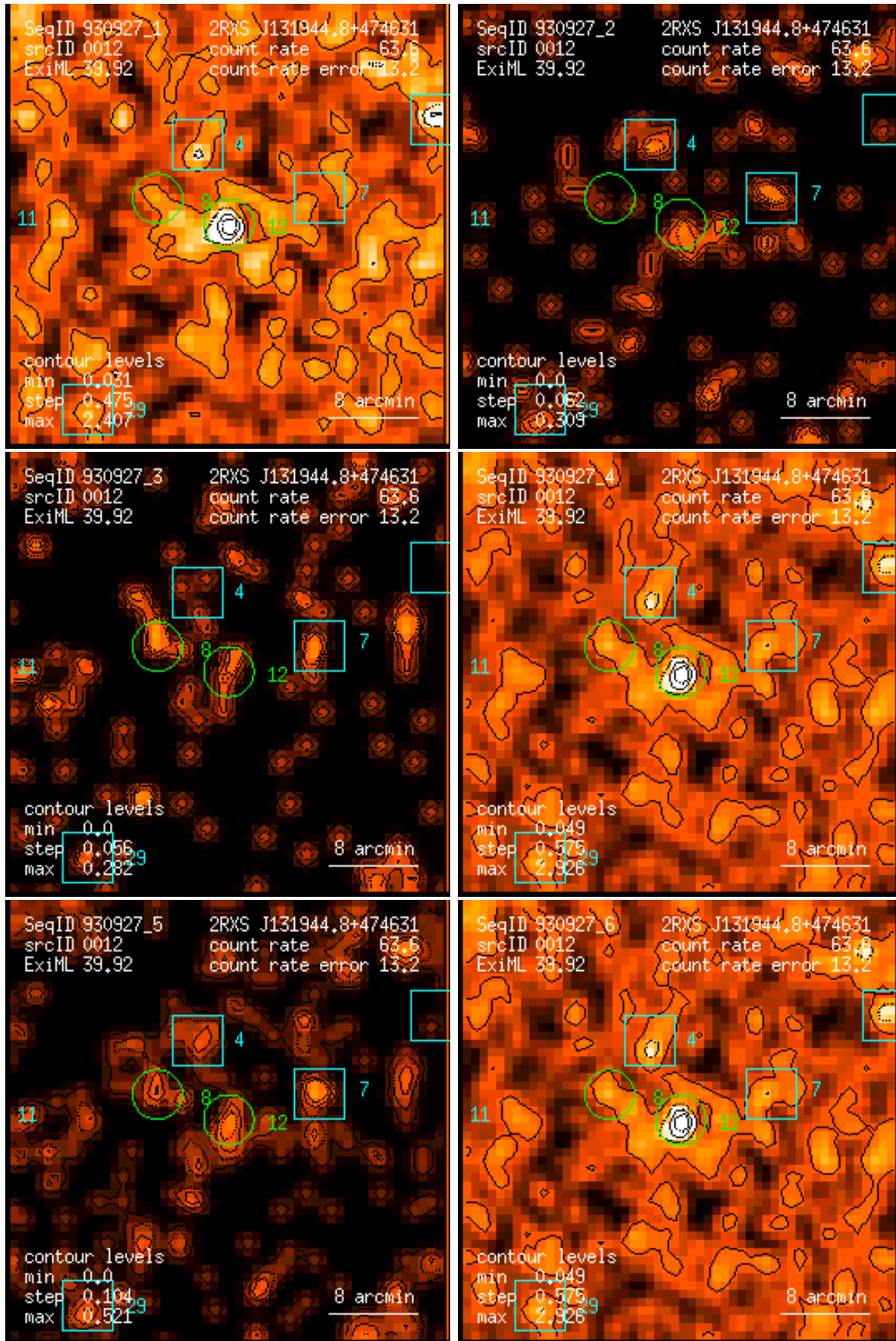
Figure 12: RASS 930927: detection 0012: band rate images, Gaussian filter: (1) PSPC channels 11 – 41, (2) 52 – 90, (3) 91 – 201, (4) 11 – 235, (5) 52 – 201, (6) 11 – 201. Broad band rates in counts/ks. Band rate contour levels in counts/ks/arcmin 2 .
