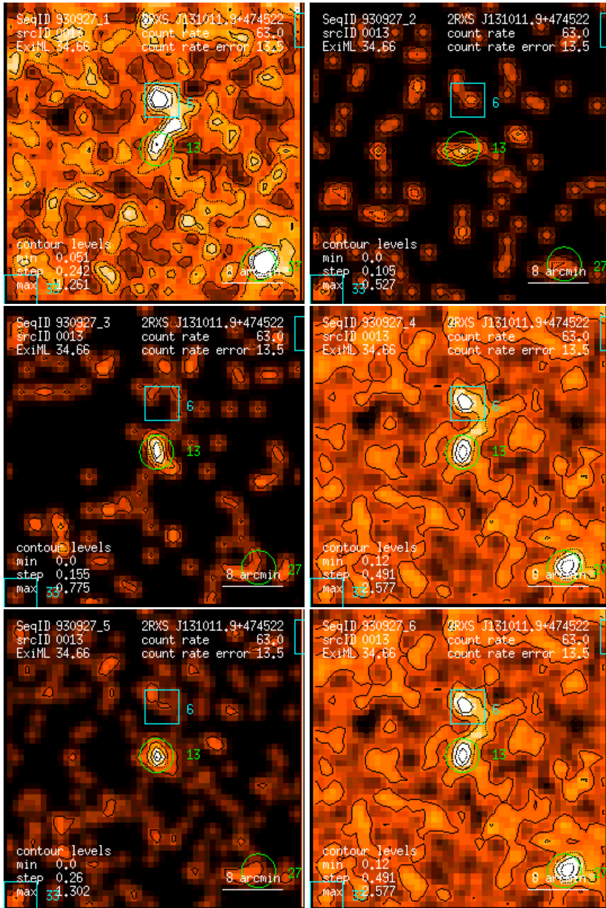
Figure 13: RASS 930927: detection 0013: band rate images, Gaussian filter: (1) PSPC channels 11 – 41, (2) 52 – 90, (3) 91 – 201, (4) 11 – 235, (5) 52 – 201, (6) 11 – 201. Broad band rates in counts/ks. Band rate contour levels in counts/ks/arcmin 2 .
