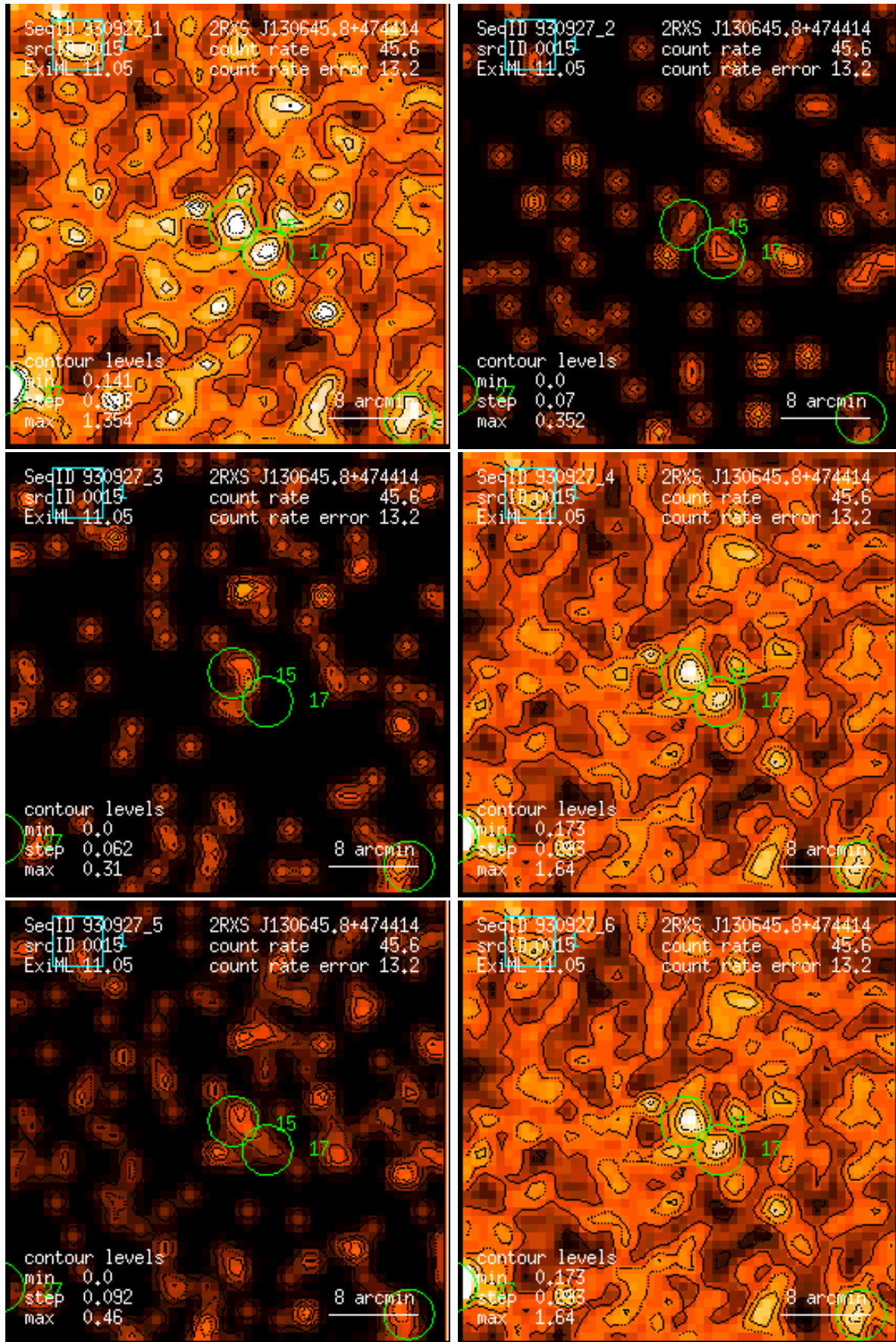
Figure 15: RASS 930927: detection 0015: band rate images, Gaussian filter: (1) PSPC channels 11 – 41, (2) 52 – 90, (3) 91 – 201, (4) 11 – 235, (5) 52 – 201, (6) 11 – 201. Broad band rates in counts/ks. Band rate contour levels in counts/ks/arcmin 2 .
