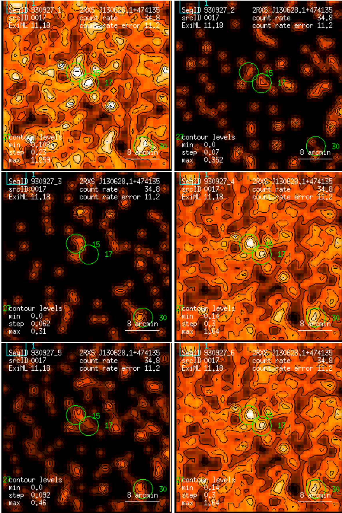
Figure 17: RASS 930927: detection 0017: band rate images, Gaussian filter: (1) PSPC channels 11 – 41, (2) 52 – 90, (3) 91 – 201, (4) 11 – 235, (5) 52 – 201, (6) 11 – 201. Broad band rates in counts/ks. Band rate contour levels in counts/ks/arcmin 2 .
