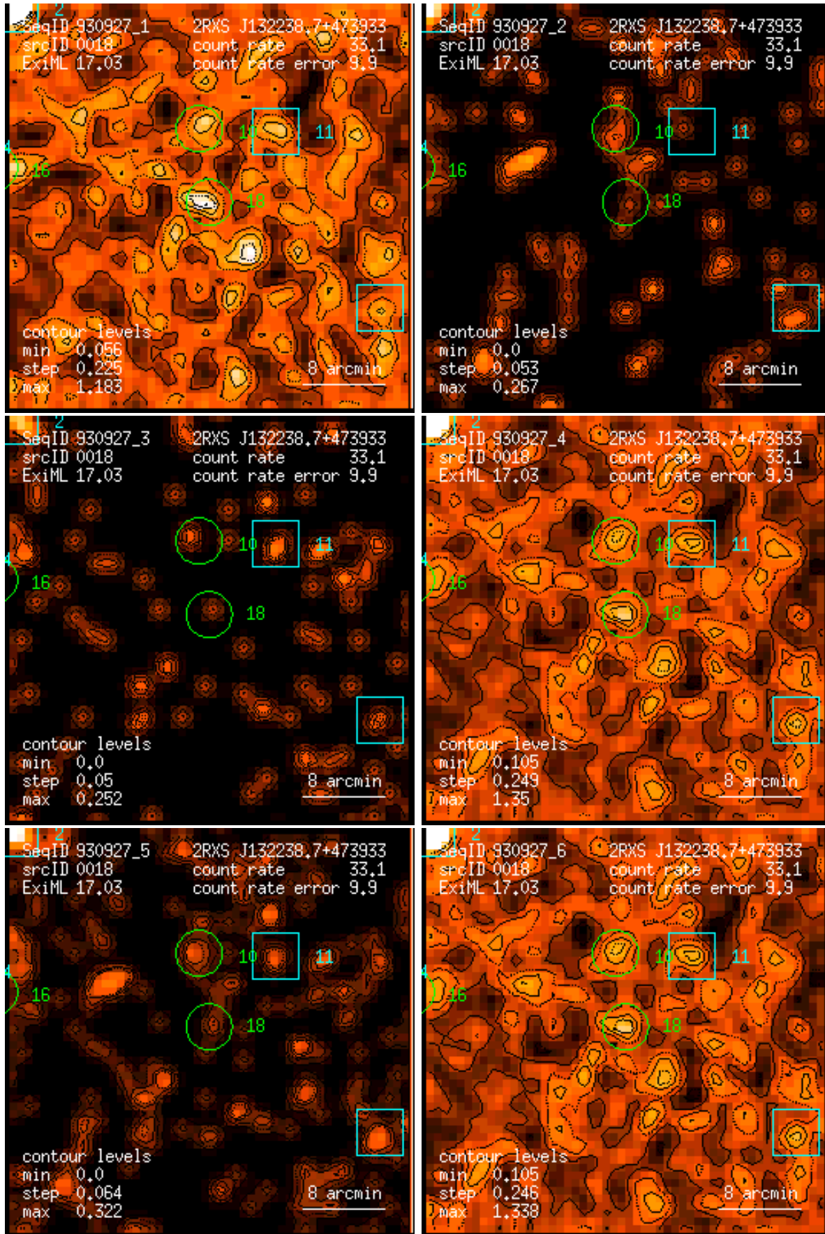
Figure 18: RASS 930927: detection 0018: band rate images, Gaussian filter: (1) PSPC channels 11 – 41, (2) 52 – 90, (3) 91 – 201, (4) 11 – 235, (5) 52 – 201, (6) 11 – 201. Broad band rates in counts/ks. Band rate contour levels in counts/ks/arcmin 2 .
