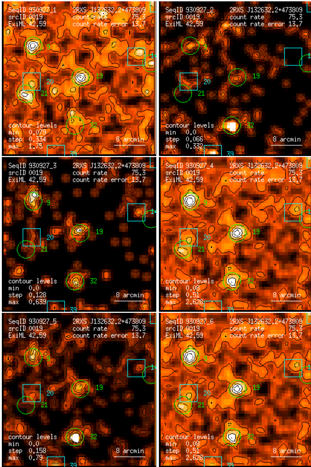
Figure 19: RASS 930927: detection 0019: band rate images, Gaussian filter: (1) PSPC channels 11 – 41, (2) 52 – 90, (3) 91 – 201, (4) 11 – 235, (5) 52 – 201, (6) 11 – 201. Broad band rates in counts/ks. Band rate contour levels in counts/ks/arcmin 2 .
