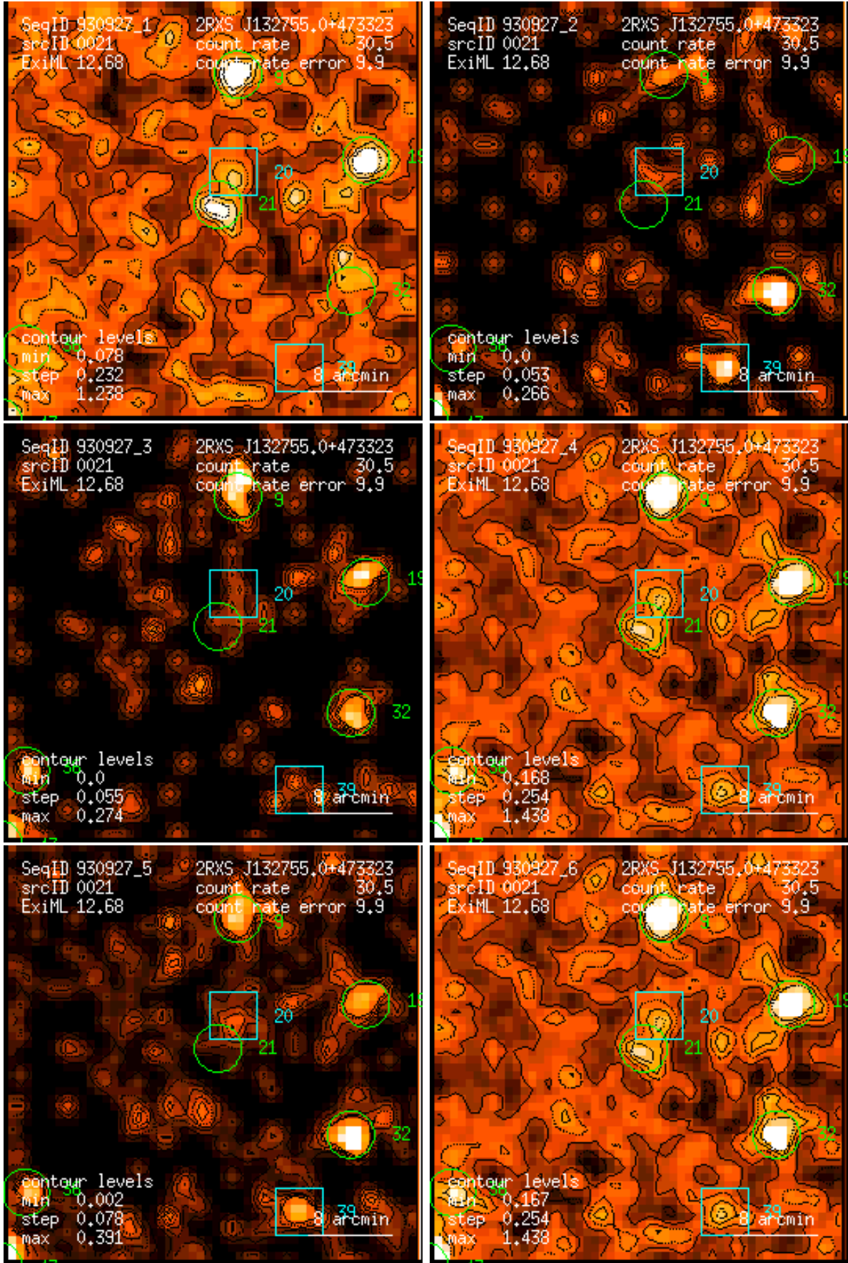
Figure 21: RASS 930927: detection 0021: band rate images, Gaussian filter: (1) PSPC channels 11 – 41, (2) 52 – 90, (3) 91 – 201, (4) 11 – 235, (5) 52 – 201, (6) 11 – 201. Broad band rates in counts/ks. Band rate contour levels in counts/ks/arcmin 2 .
