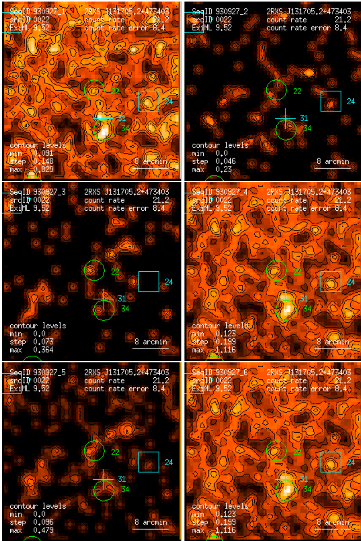
Figure 22: RASS 930927: detection 0022: band rate images, Gaussian filter: (1) PSPC channels 11 – 41, (2) 52 – 90, (3) 91 – 201, (4) 11 – 235, (5) 52 – 201, (6) 11 – 201. Broad band rates in counts/ks. Band rate contour levels in counts/ks/arcmin 2 .
