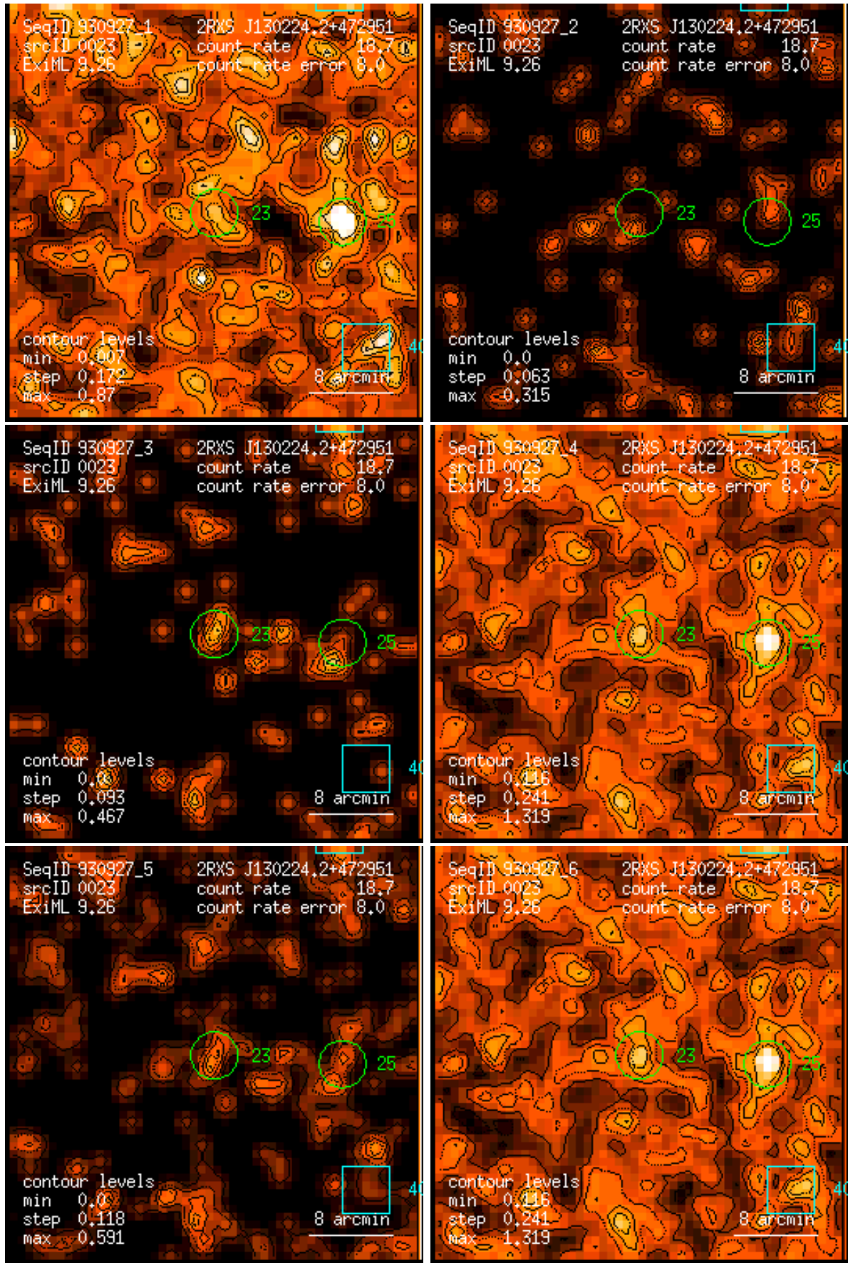
Figure 23: RASS 930927: detection 0023: band rate images, Gaussian filter: (1) PSPC channels 11 – 41, (2) 52 – 90, (3) 91 – 201, (4) 11 – 235, (5) 52 – 201, (6) 11 – 201. Broad band rates in counts/ks. Band rate contour levels in counts/ks/arcmin 2 .
