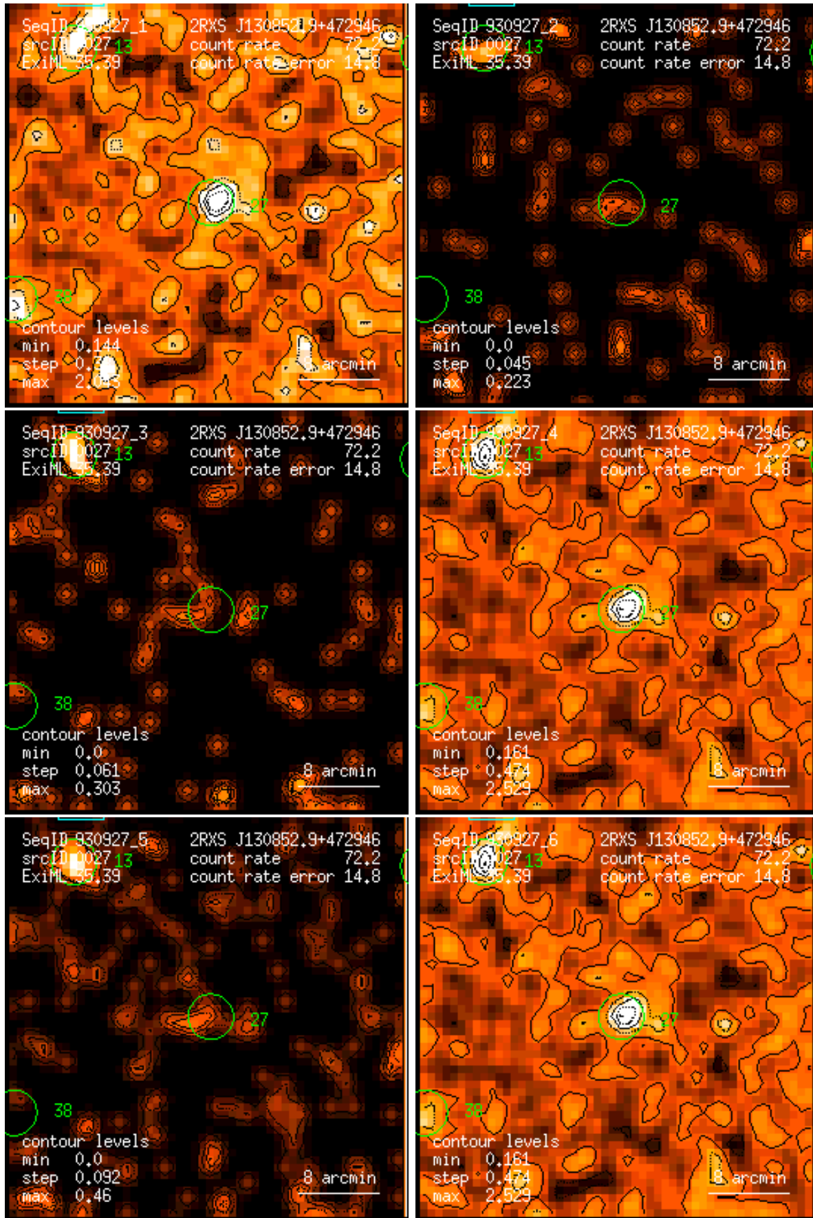
Figure 27: RASS 930927: detection 0027: band rate images, Gaussian filter: (1) PSPC channels 11 – 41, (2) 52 – 90, (3) 91 – 201, (4) 11 – 235, (5) 52 – 201, (6) 11 – 201. Broad band rates in counts/ks. Band rate contour levels in counts/ks/arcmin 2 .
