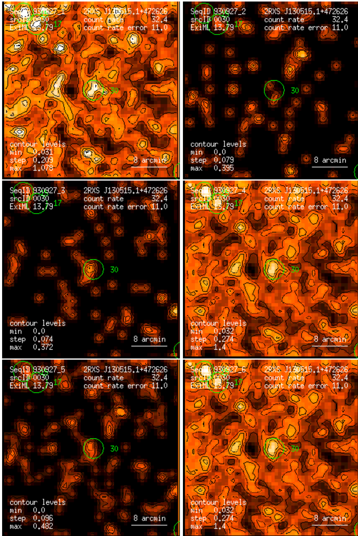
Figure 30: RASS 930927: detection 0030: band rate images, Gaussian filter: (1) PSPC channels 11 – 41, (2) 52 – 90, (3) 91 – 201, (4) 11 – 235, (5) 52 – 201, (6) 11 – 201. Broad band rates in counts/ks. Band rate contour levels in counts/ks/arcmin 2 .
