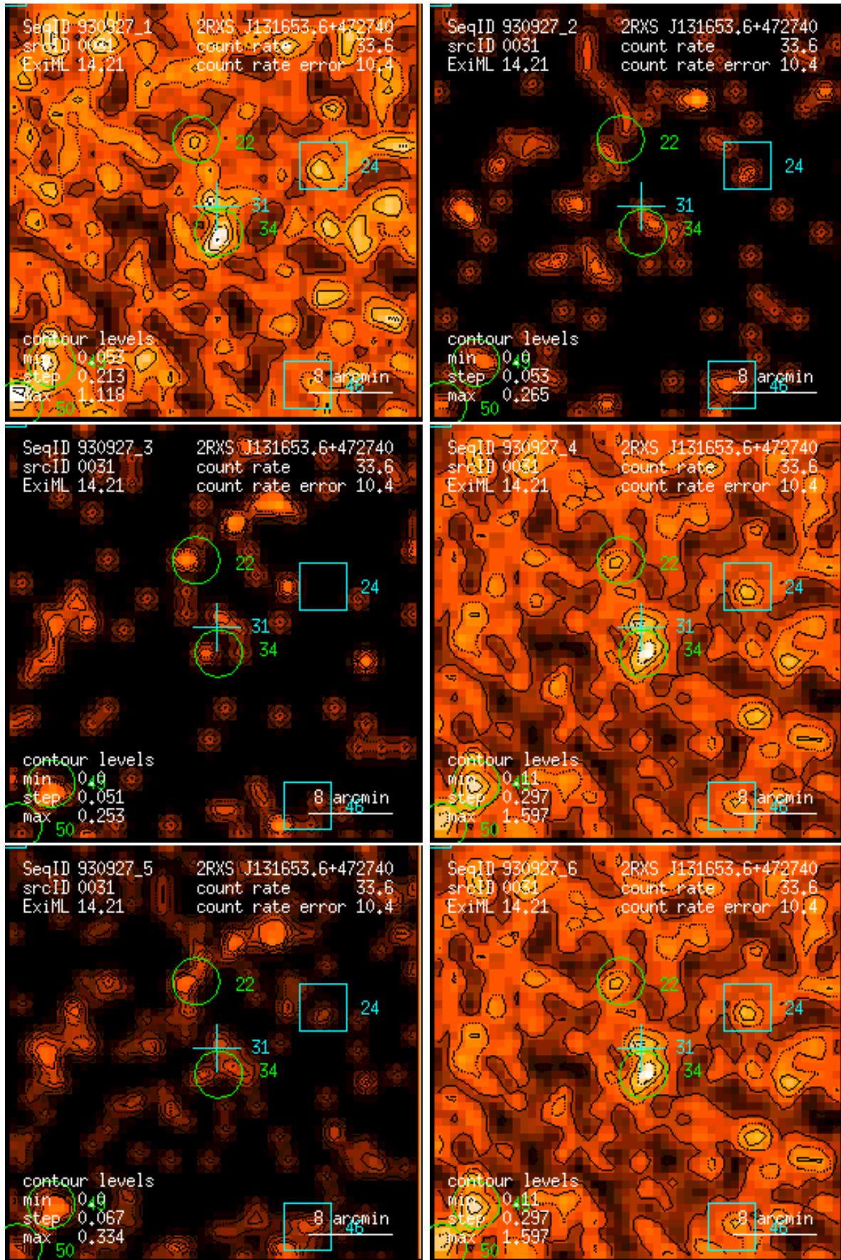
Figure 31: RASS 930927: detection 0031: band rate images, Gaussian filter: (1) PSPC channels 11 – 41, (2) 52 – 90, (3) 91 – 201, (4) 11 – 235, (5) 52 – 201, (6) 11 – 201. Broad band rates in counts/ks. Band rate contour levels in counts/ks/arcmin 2 .
