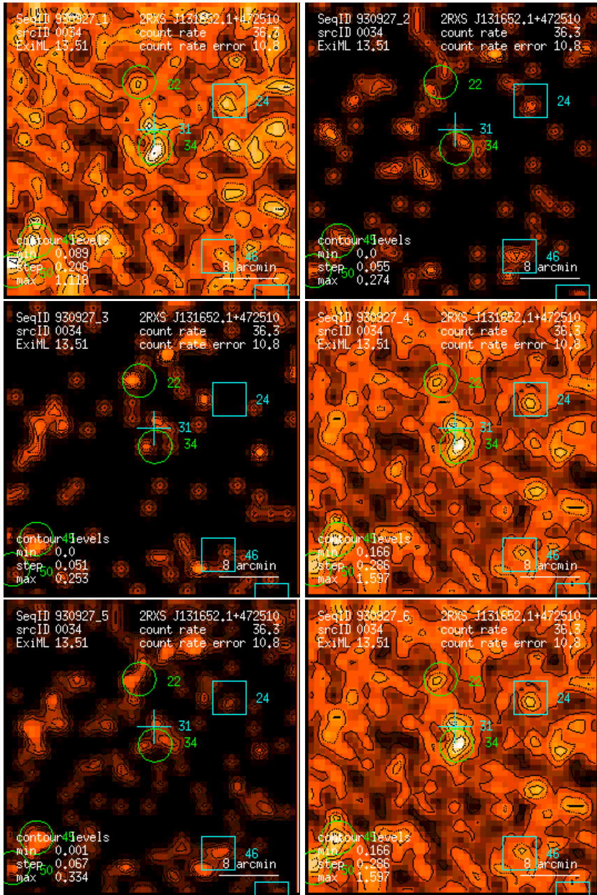
Figure 34: RASS 930927: detection 0034: band rate images, Gaussian filter: (1) PSPC channels 11 – 41, (2) 52 – 90, (3) 91 – 201, (4) 11 – 235, (5) 52 – 201, (6) 11 – 201. Broad band rates in counts/ks. Band rate contour levels in counts/ks/arcmin 2 .
