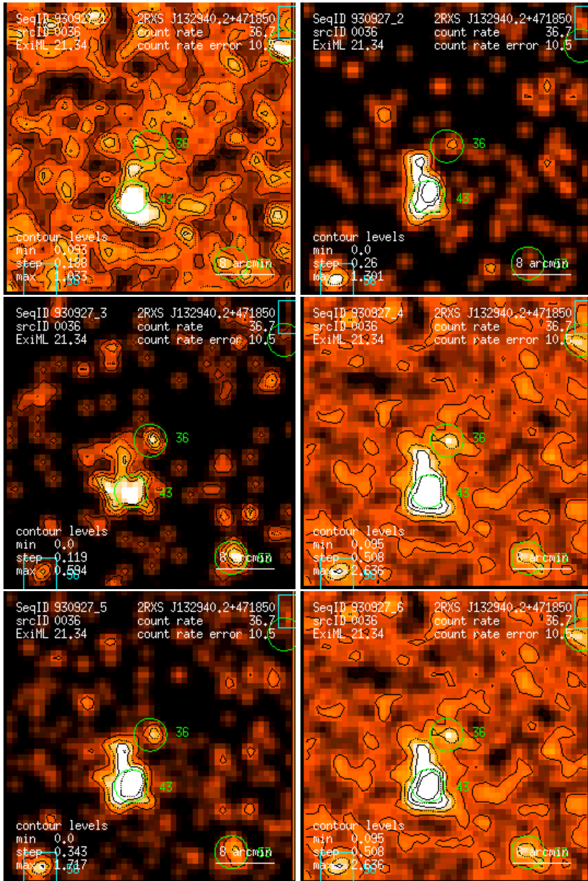
Figure 36: RASS 930927: detection 0036: band rate images, Gaussian filter: (1) PSPC channels 11 – 41, (2) 52 – 90, (3) 91 – 201, (4) 11 – 235, (5) 52 – 201, (6) 11 – 201. Broad band rates in counts/ks. Band rate contour levels in counts/ks/arcmin 2 .
