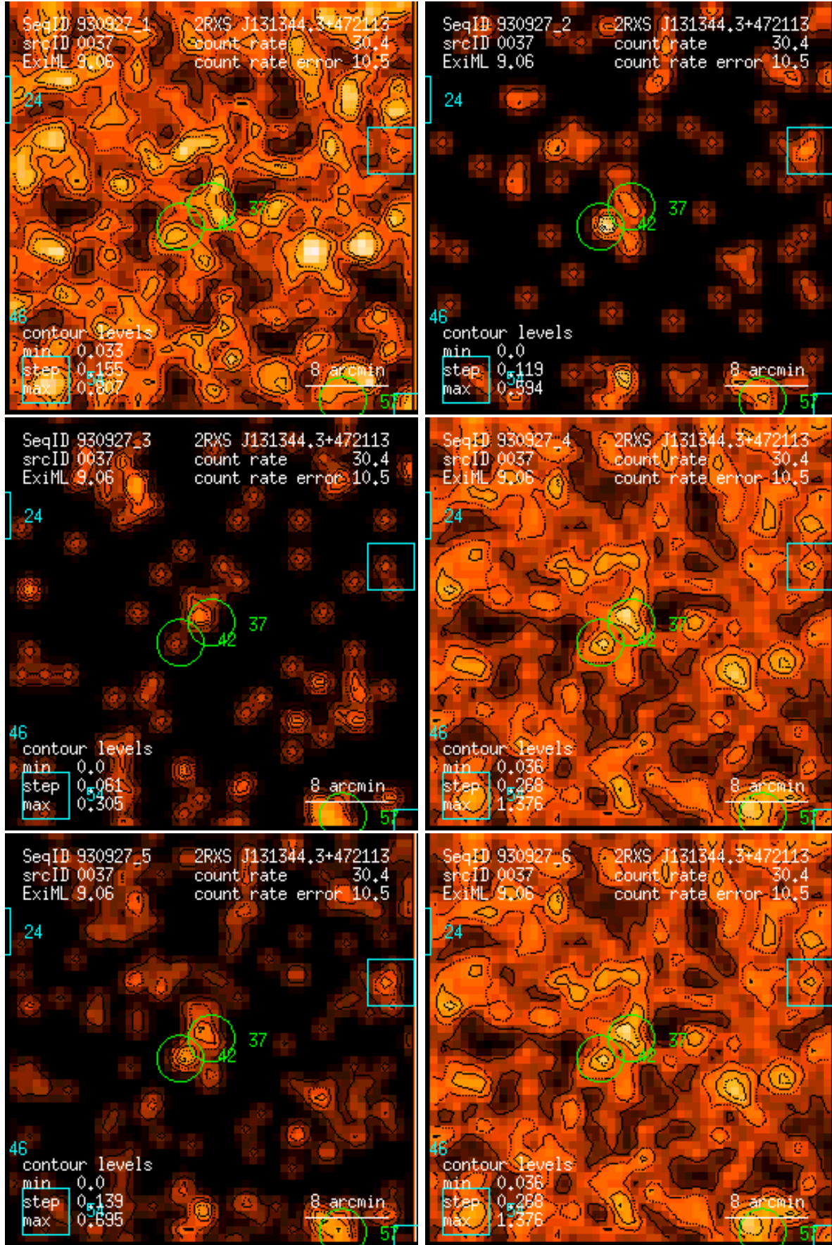
Figure 37: RASS 930927: detection 0037: band rate images, Gaussian filter: (1) PSPC channels 11 – 41, (2) 52 – 90, (3) 91 – 201, (4) 11 – 235, (5) 52 – 201, (6) 11 – 201. Broad band rates in counts/ks. Band rate contour levels in counts/ks/arcmin 2 .
