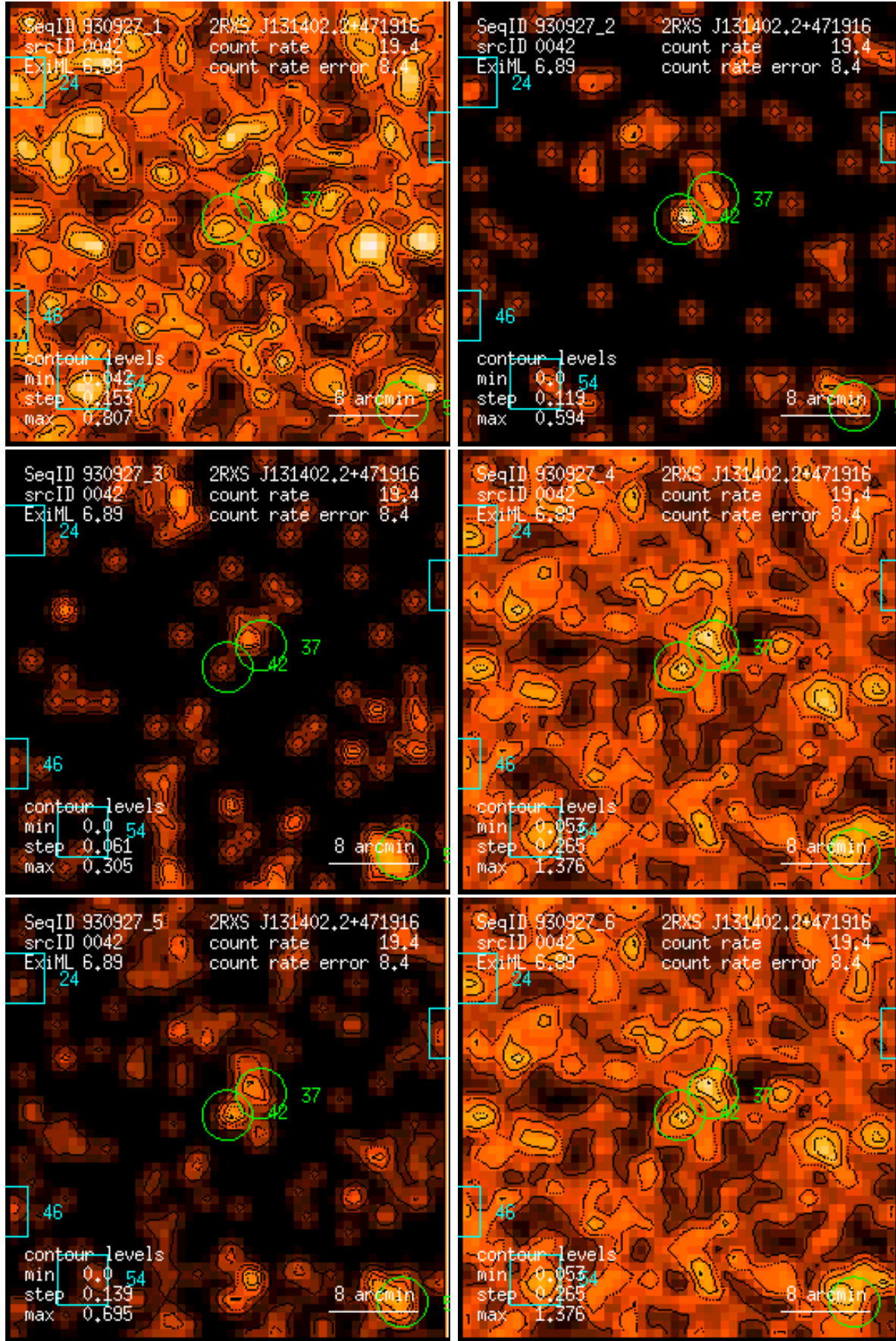
Figure 42: RASS 930927: detection 0042: band rate images, Gaussian filter: (1) PSPC channels 11 – 41, (2) 52 – 90, (3) 91 – 201, (4) 11 – 235, (5) 52 – 201, (6) 11 – 201. Broad band rates in counts/ks. Band rate contour levels in counts/ks/arcmin 2 .
