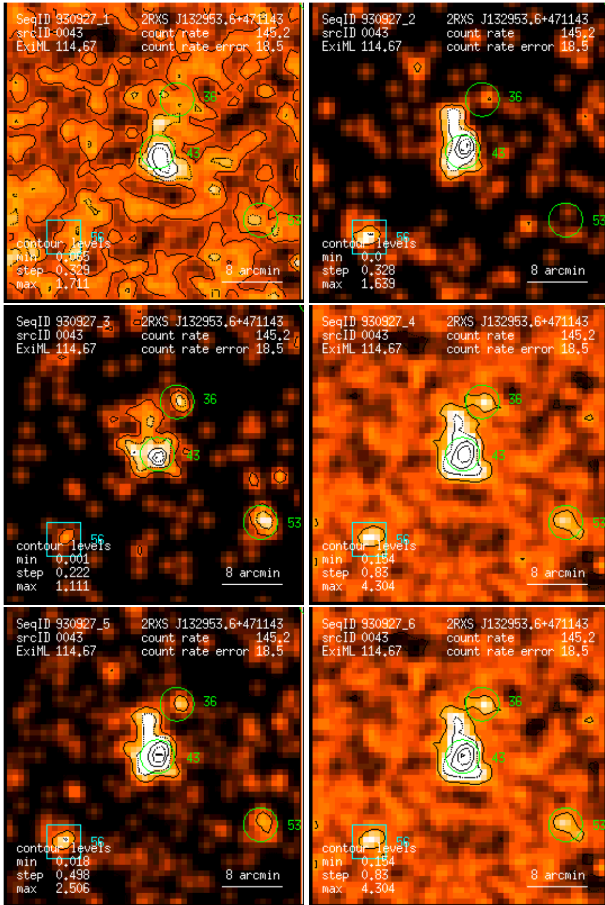
Figure 43: RASS 930927: detection 0043: band rate images, Gaussian filter: (1) PSPC channels 11 – 41, (2) 52 – 90, (3) 91 – 201, (4) 11 – 235, (5) 52 – 201, (6) 11 – 201. Broad band rates in counts/ks. Band rate contour levels in counts/ks/arcmin 2 .
