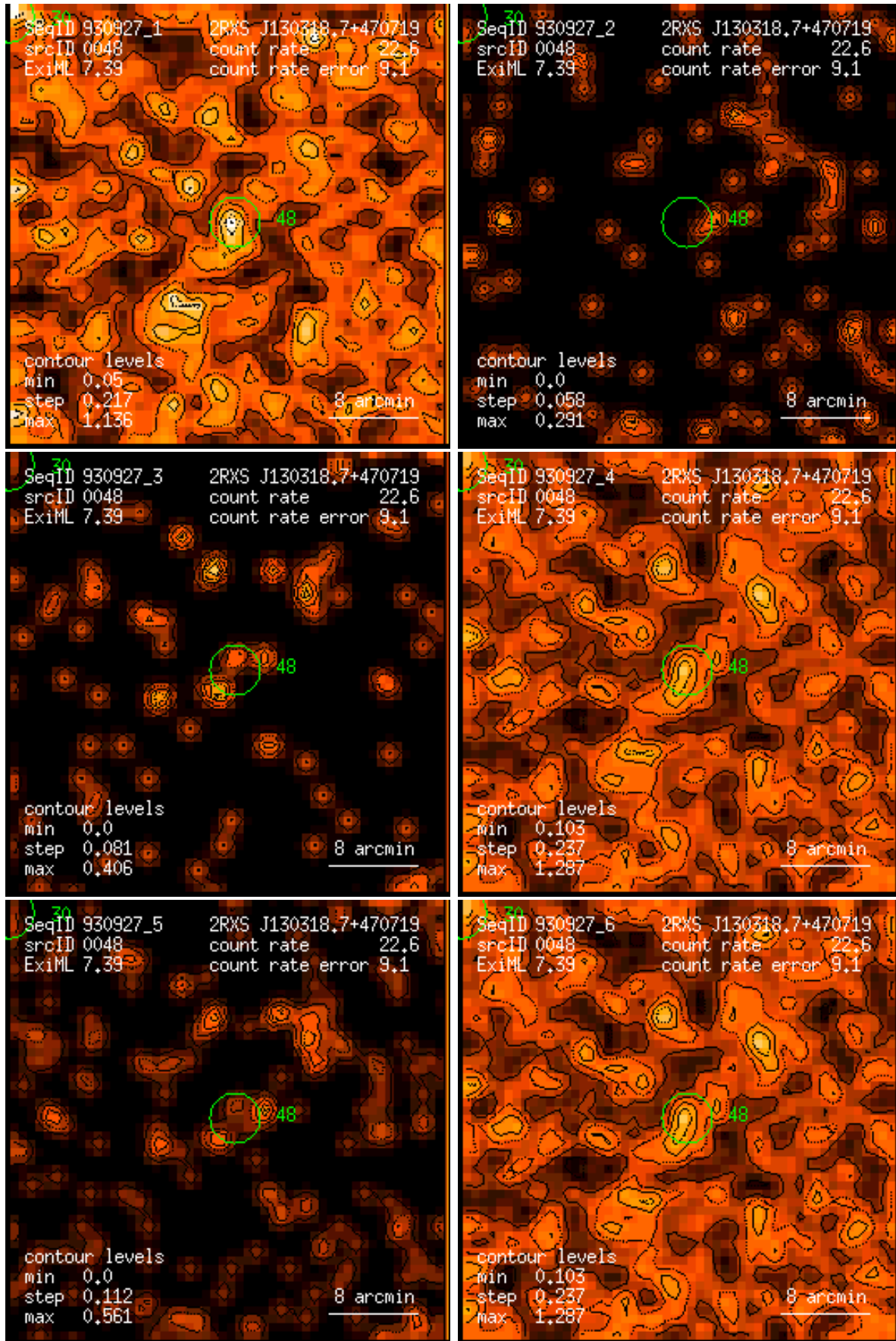
Figure 48: RASS 930927: detection 0048: band rate images, Gaussian filter: (1) PSPC channels 11 – 41, (2) 52 – 90, (3) 91 – 201, (4) 11 – 235, (5) 52 – 201, (6) 11 – 201. Broad band rates in counts/ks. Band rate contour levels in counts/ks/arcmin 2 .
