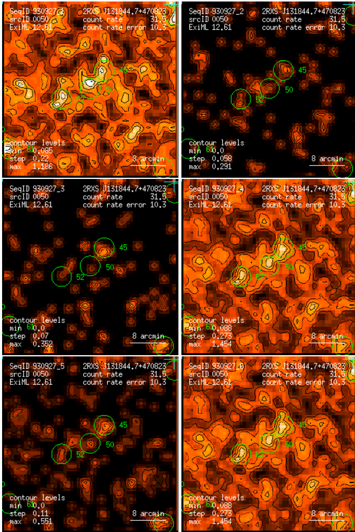
Figure 50: RASS 930927: detection 0050: band rate images, Gaussian filter: (1) PSPC channels 11 – 41, (2) 52 – 90, (3) 91 – 201, (4) 11 – 235, (5) 52 – 201, (6) 11 – 201. Broad band rates in counts/ks. Band rate contour levels in counts/ks/arcmin 2 .
