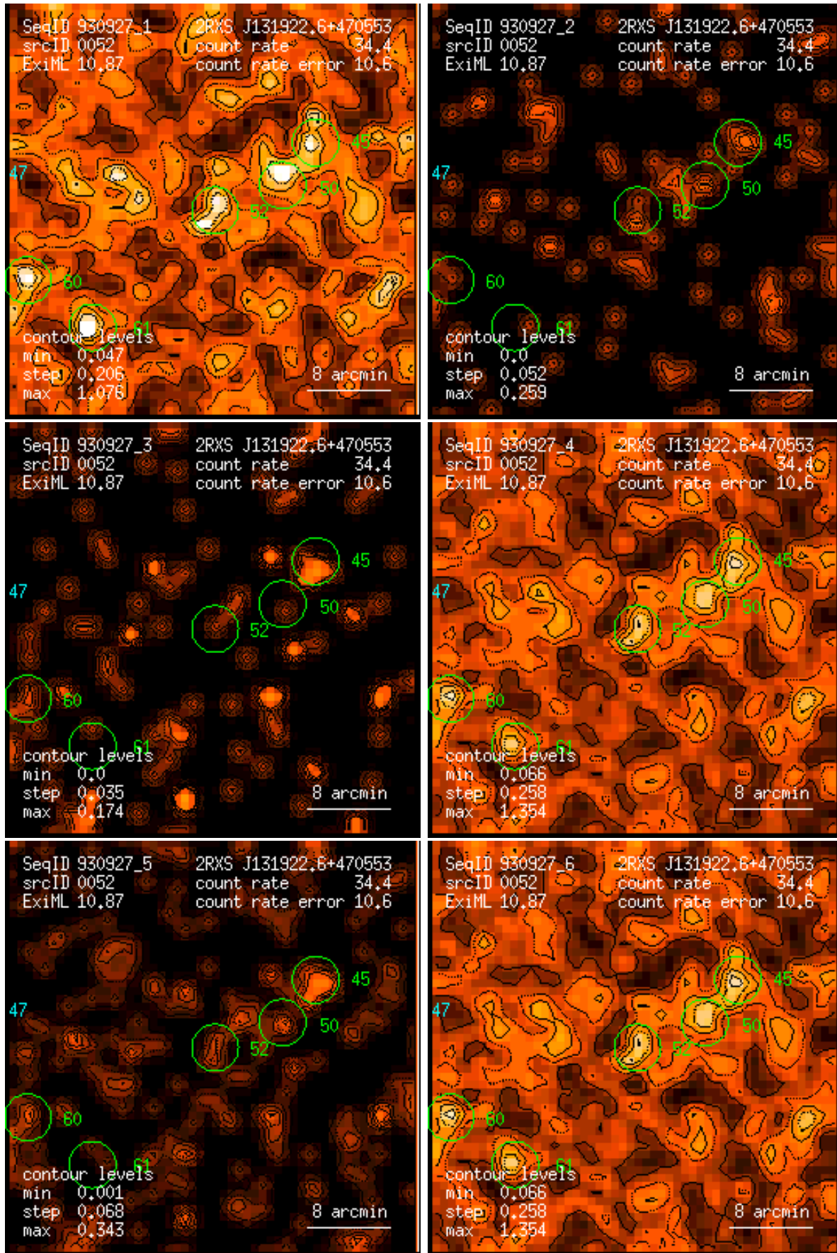
Figure 52: RASS 930927: detection 0052: band rate images, Gaussian filter: (1) PSPC channels 11 – 41, (2) 52 – 90, (3) 91 – 201, (4) 11 – 235, (5) 52 – 201, (6) 11 – 201. Broad band rates in counts/ks. Band rate contour levels in counts/ks/arcmin 2 .
