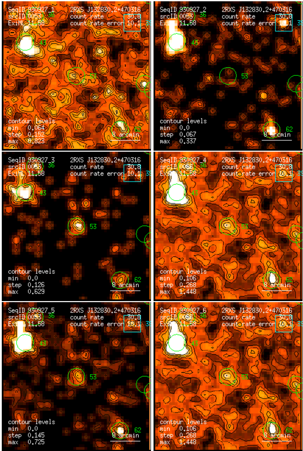
Figure 53: RASS 930927: detection 0053: band rate images, Gaussian filter: (1) PSPC channels 11 – 41, (2) 52 – 90, (3) 91 – 201, (4) 11 – 235, (5) 52 – 201, (6) 11 – 201. Broad band rates in counts/ks. Band rate contour levels in counts/ks/arcmin 2 .
