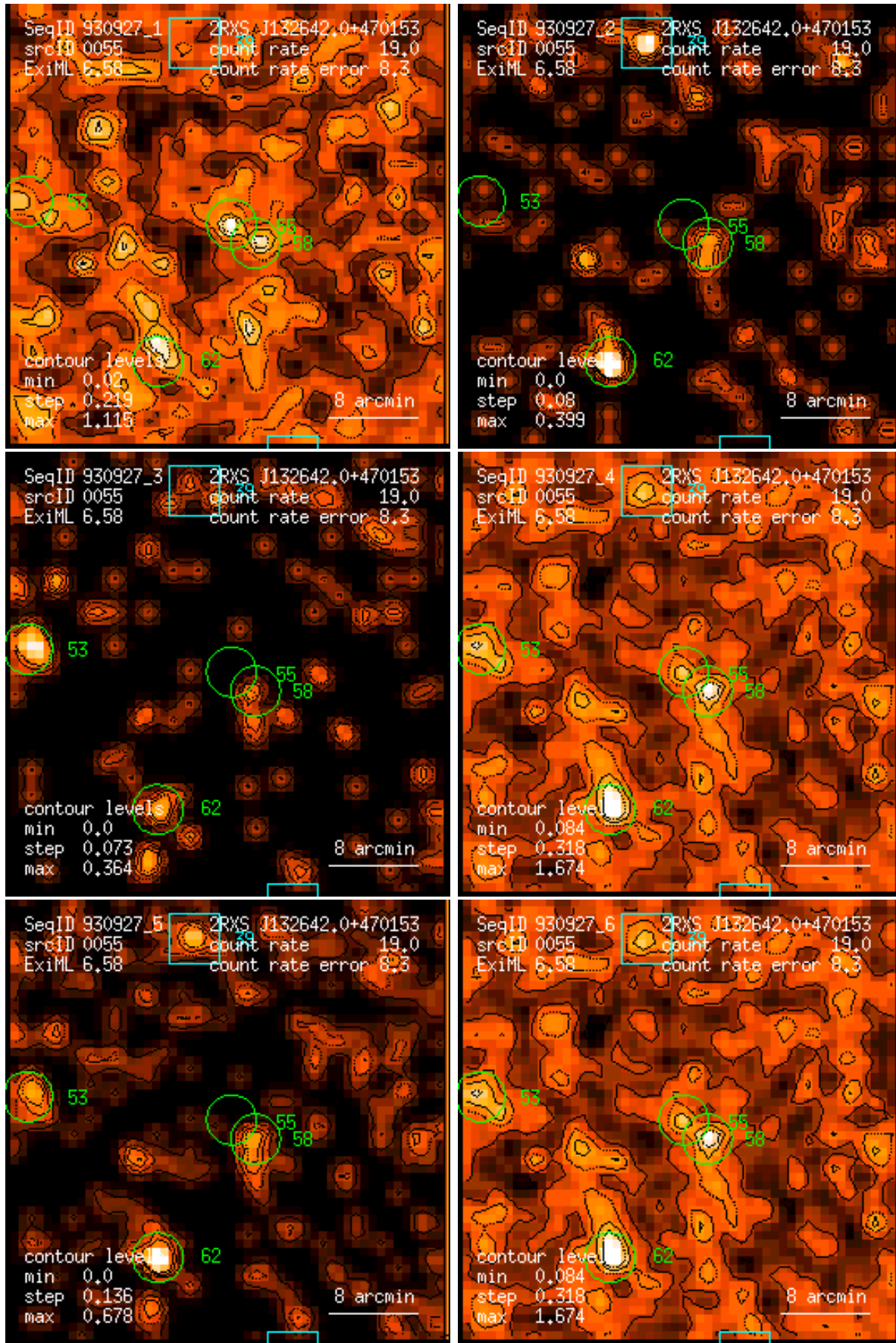
Figure 55: RASS 930927: detection 0055: band rate images, Gaussian filter: (1) PSPC channels 11 – 41, (2) 52 – 90, (3) 91 – 201, (4) 11 – 235, (5) 52 – 201, (6) 11 – 201. Broad band rates in counts/ks. Band rate contour levels in counts/ks/arcmin 2 .
