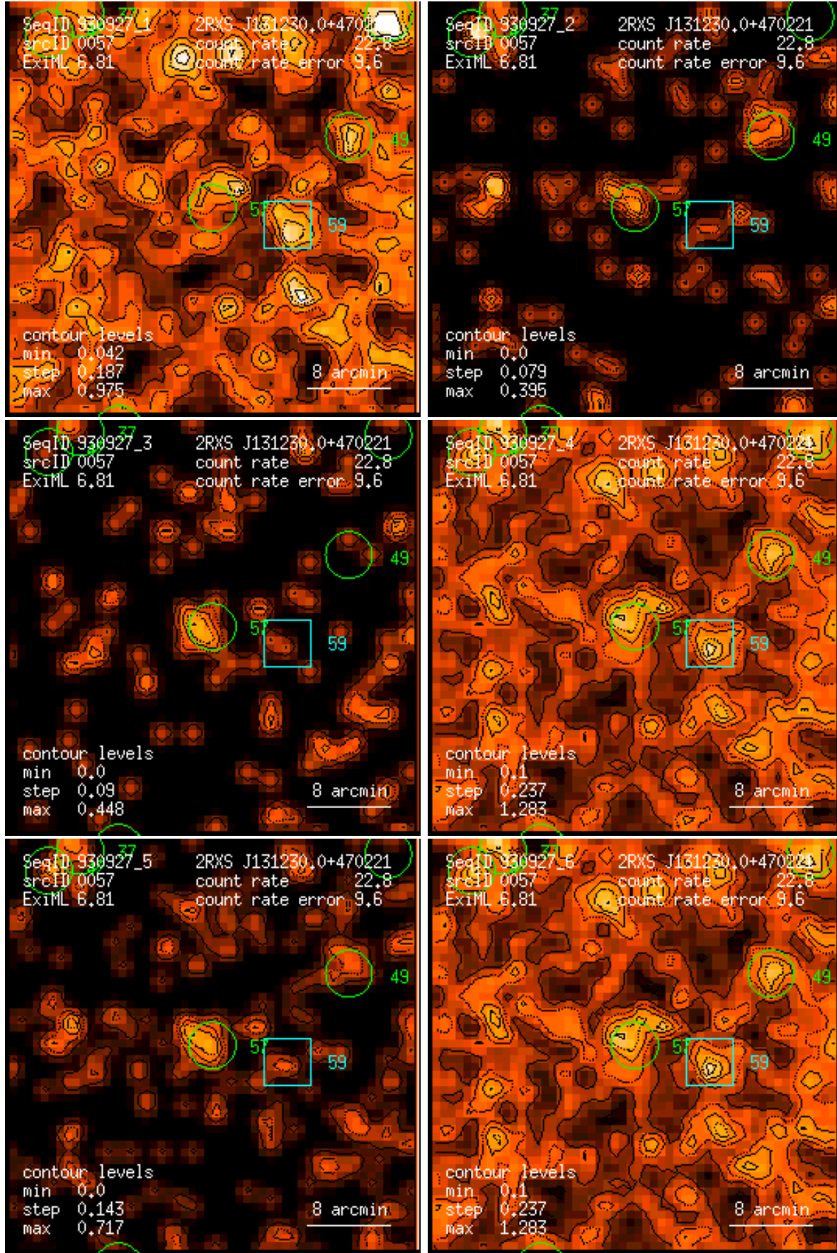
Figure 57: RASS 930927: detection 0057: band rate images, Gaussian filter: (1) PSPC channels 11 – 41, (2) 52 – 90, (3) 91 – 201, (4) 11 – 235, (5) 52 – 201, (6) 11 – 201. Broad band rates in counts/ks. Band rate contour levels in counts/ks/arcmin 2 .
